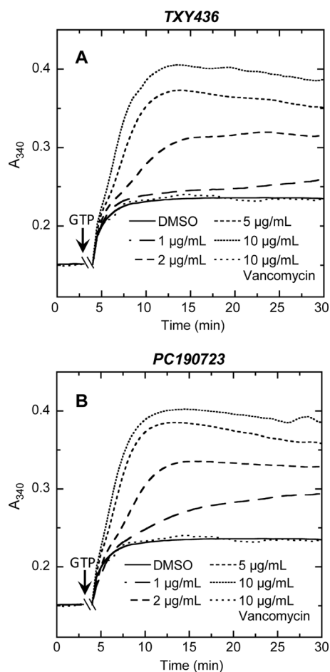
FIG 6 Concentration dependence of the impact of TXY436 (A) or PC190723 (B) on the polymerization of S. aureus FtsZ, as determined by monitoring time-dependent changes in absorbance at 340 nm ( A_{340} ) at 25°C. The time-dependent A_{340} polymerization profiles were acquired in the presence of DMSO (solvent control) or the indicated concentrations of compound (ranging from 1 to 10 \mu\text{g/ml} ). The polymerization profile acquired in the presence of vancomycin at 10 \mu\text{g/ml} is also included as a negative (non-FtsZ-targeting) control. Experimental conditions for the polymerization studies were 5 \mu\text{M} FtsZ, 50 mM Tris-HCl (pH 7.4), 50 mM KCl, and 10 mM magnesium acetate. Polymerization reactions were initiated by the addition of 4 mM GTP at the times indicated by the arrows.
