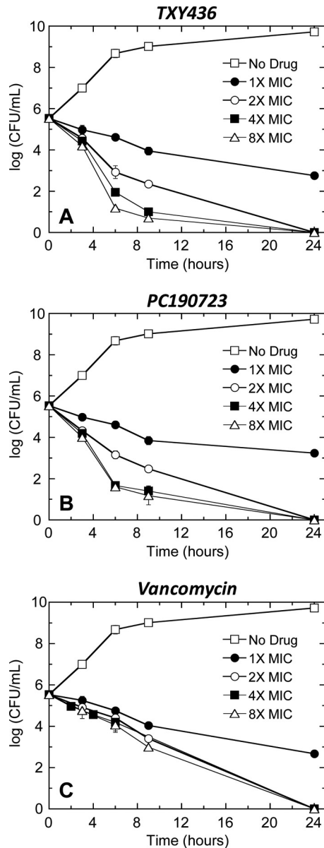
FIG 4 Time-kill curves for S. aureus 8325-4 (MSSA). Each data point reflects the average of two independent measurements, with the error bars reflecting the standard deviation from the mean. Bacteria were treated with DMSO vehicle only (no drug), TXY436 (A), PC190723 (B), or vancomycin (C). All agents were used at concentrations ranging from 1× to 8× the MIC.
