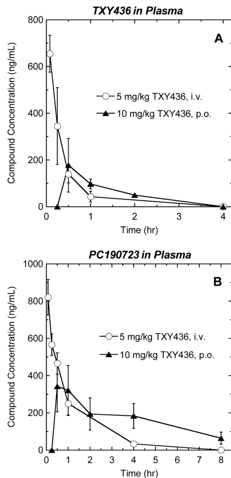
FIG 8 Time-dependent plasma concentrations of TXY436 (A) and PC190723 (B) after a single i.v. administration of TXY436 at 5 mg/kg (○) or a single p.o. administration of TXY436 at 10 mg/kg (▲) to male BALB/c mice.
