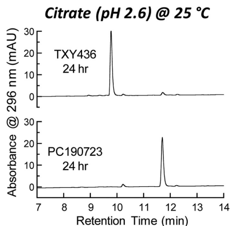
FIG 2 Reverse-phase HPLC chromatograms of TXY436 and PC190723 after incubation for 24 h in 10 mM citrate (pH 2.6) at 25°C. The concentration of each compound was 10 μg/ml.
