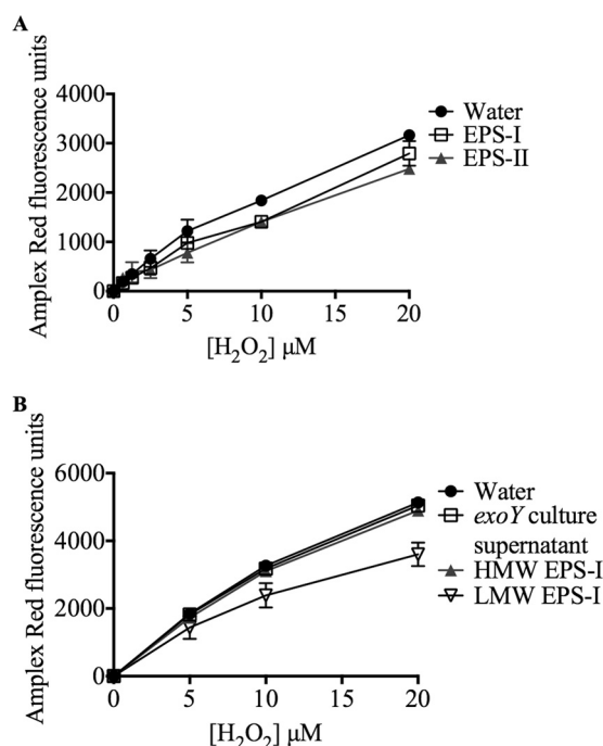
FIG 5 Exopolysaccharides decrease H 2 O 2 concentrations in vitro . (A) Amount of H 2 O 2 detected by Amplex Red when incubated with 7 µg EPS-I (open squares) or 7 µg EPS-II (filled triangles). (b) Amplex Red detection of H 2 O 2 incubated with either the culture supernatant from the exoY strain (open squares), 25 µg HMW EPS-I (filled triangles), or 20 µg LMW EPS-I (open inverted triangles). Error bars indicate standard deviations (not visible in all data points due to small errors).
