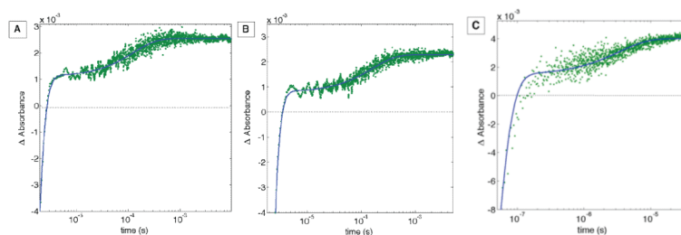
Figure 5. Transient absorption traces (630 nm) for RuH107NO 2 YO - 109 (A), RuH126NO 2 YO - 122 (B) and RuH124NO 2 YO - 122 (C) azurins. Kinetics traces are fit as described in the experimental section. The apparent bleach at very early times is due to residual luminescence from *Ru. The concentration of Ru(NH 3 ) 6 Cl 3 was 12 mM in each sample.
