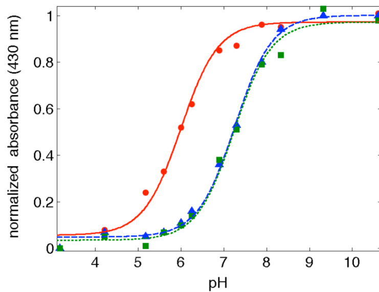
Figure 2. Titration curves for: H107NO 2 YOH109 (red ●); H124NO 2 YOH122 (green ■) and H126NO 2 YOH122 (blue ▲). The lines are fits as described in Methods.
