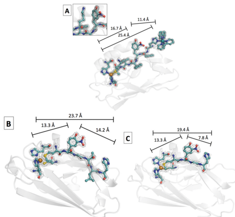
Figure 4. Structures of the electron transfer units of RuH107NO 2 YO - 109 (PDB 4HHG, 1.6 Å) (A); H126NO 2 YOH122 (PDB 4HIP, 1.9 Å) (B), and H124NO 2 YOH122 (PDB 4HHW, 2.0 Å) (C) azurins. The peptide chain connecting the Ru-label, NO 2 YOH, and azurin-Cu is shown in cyan and the rest of the protein is shown as a gray ribbon. The distances between redox centers (see text) are shown above the black bars; the bars are not intended to show angles between cofactors. The inset in (A) shows Lys122. The Lys122(N) to NO 2 YO(O phenolate ) distance is 4.3 Å. Cu 2+ is depicted as an orange sphere and Ru 2+ in (A) is a turquoise sphere.
