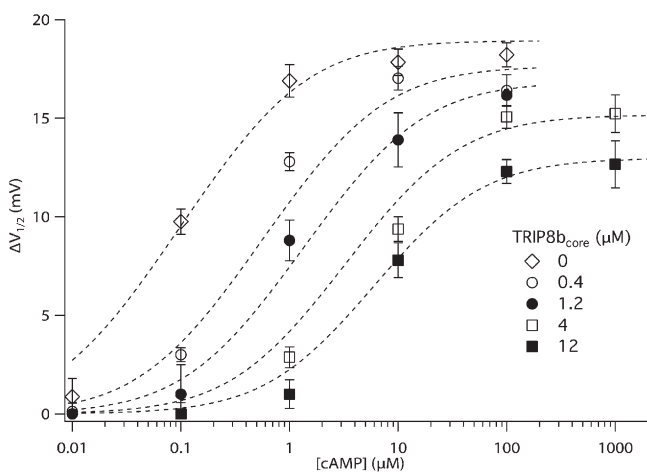
Figure 7. \Delta V_{1/2} as a function of [\text{cAMP}] and [\text{TRIP8b}_{\text{core}}] polypeptide, fitted by the 12-state allosteric model. The \text{TRIP8b}_{\text{core}} polypeptide concentrations are indicated. The parameters of the front face of the model (corresponding to the six-state cyclic model) are adopted from Zhou and Siegelbaum (2007): L = 0.43 , s = 4.4 , K_C^A = 0.844 \mu\text{M} , K_O^A = 0.008 \mu\text{M} . The best fit of the model yields the following values for the other parameters: K_C^T = 0.089 \pm 0.027 \mu\text{M} , K_O^T = 0.064 \pm 0.010 \mu\text{M} , K_{TC}^A = 33.58 \pm 8.18 \mu\text{M} , K_{TO}^A = 3.53 \pm 1.33 \mu\text{M} . K_{AC}^T and K_{AO}^T are then derived from the other parameters: K_{AC}^T = K_{TC}^A \cdot K_C^T / K_C^A = 3.54 \mu\text{M} and K_{AO}^T = K_{TO}^A \cdot K_O^T / K_O^A = 28.24 \mu\text{M} . Error bars show SEM. See supplemental text for further details.
