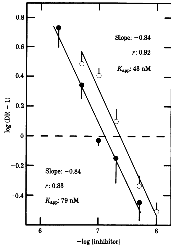
FIG. 4. Effect of pimoziide and fluspirilene on potassium-induced calcium-dependent contractions of rat vas deferens. The inhibition of CaCl 2 -dependent contractions of vasa deferentia depolarized by 80 mM KCl was plotted by the method of Schild (24). For each estimation, CaCl 2 was added at 2 min intervals. Three estimations were made to obtain a mean for the control curve while single determinations were used for the response in the presence of fluspirilene (●) or pimoziide (○). The dose ratio (DR) is the ratio of the concentration of CaCl 2 required to elicit responses equal to 50% of the maximum control response observed. Each point represents mean ± SEM ( n = 6). Fluspirilene gave a slope of -0.84, a correlation coefficient ( r ) of 0.83, and K app = 79 nM; pimoziide gave a slope of -0.84, r = 0.92, and K app = 0.43 nM. These slopes are consistent with competitive interaction.
