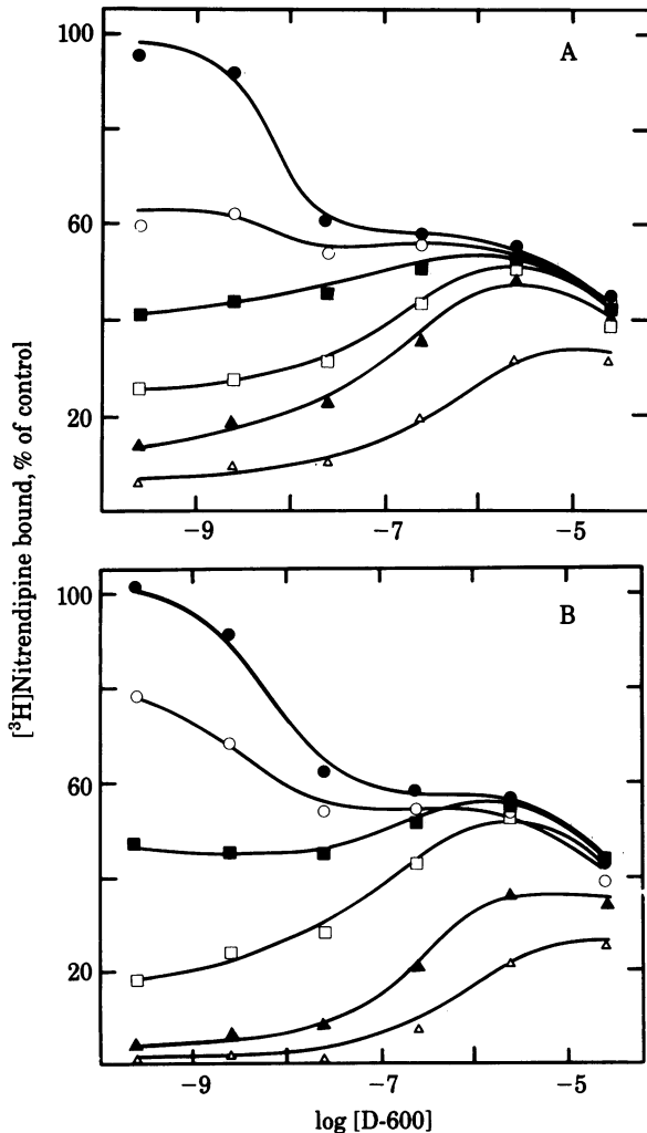
FIG. 3. Methoxyverapamil (D-600) reverses the inhibition of [ 3 H]nitrendipine binding produced by fluspirilene (A) or pimoziide (B). Dose-response curves for the influence of D-600 on [ 3 H]nitrendipine binding to membranes were obtained with six concentrations of D-600 and 0.2 nM [ 3 H]nitrendipine. [ 3 H]Nitrendipine binding was determined at each concentration of D-600 in the absence (●) or presence of 7.5 nM (○), 25 nM (■), 75 nM (□), 250 nM (▲), or 750 nM (Δ) fluspirilene or pimoziide.
