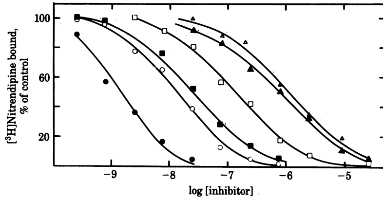
FIG. 2. Inhibition of [ 3 H]nitrendipine binding by nifedipine (●), pimoziide (○), fluspirilene (■), prenylamine (□), lidoflazine (▲), and spiperone (Δ). Dose-response curves for the inhibition of 0.2 nM [ 3 H]nitrendipine binding were constructed. Values are means of two or three experiments, each performed in triplicate.
