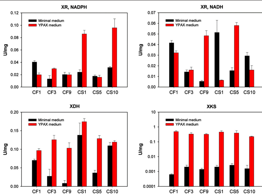
Figure 7 Enzyme activities of xylose reductase (XR), xylitol dehydrogenase (XDH), and xylulose kinase (XKS) in S. cerevisiae strains. The activities of XRs with both NADPH and NADH as the cofactors were measured.
