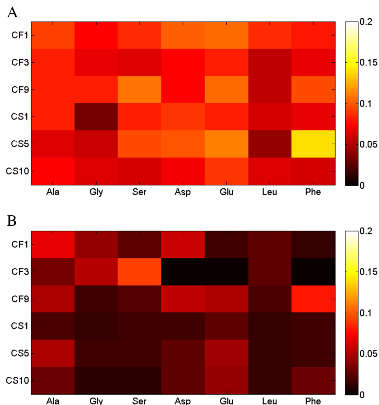
Figure 6 ^{13}\text{C} enrichment of proteinogenic amino acids in S. cerevisiae strains cultured in A) defined minimal medium and B) YPAX medium. Note: the mass spectrum of Asp, Glu and Phe in CF3 strain cultured in YPAX medium had too much noise to derive the reliable readouts of ^{13}\text{C} enrichment.
