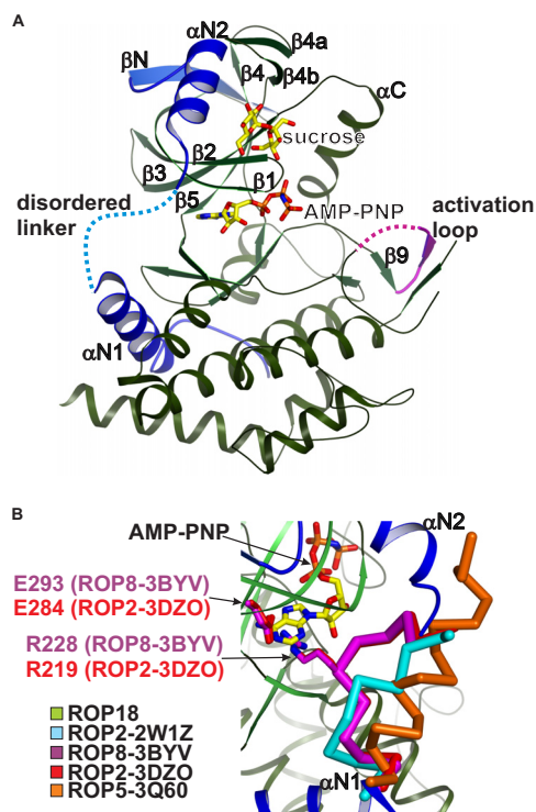
FIGURE 1. Crystal structure of the ROP18 kinase domain. A , schematic rendering of the ROP18 kinase domain with the N-terminal subdomain highlighted in blue and disordered regions indicated by dotted lines. The bound sucrose and AMP-PNP molecules are shown in stick rendering with yellow carbons. B , close-up view of the \alpha N1- \alpha N2 linker within the N-terminal subdomain. Although this linker is disordered in ROP18, in ROP2-3DZO and ROP8-3BYV the linker adopts an autoinhibitory conformation (red and purple C \alpha traces, respectively) stabilized by an Arg-Glu salt bridge (stick rendering) that precludes ATP binding. The corresponding regions from ROP2-2W1Z and ROP5-3Q60 are shown as cyan and orange C \alpha traces, respectively.
