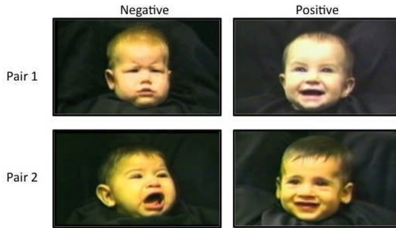
Figure 1. Photos of stimulus events
