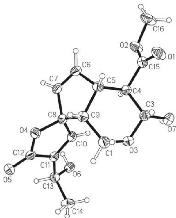
Figure 1. The molecular structure of (I), with displacement ellipsoids drawn at the 50% probability level.
