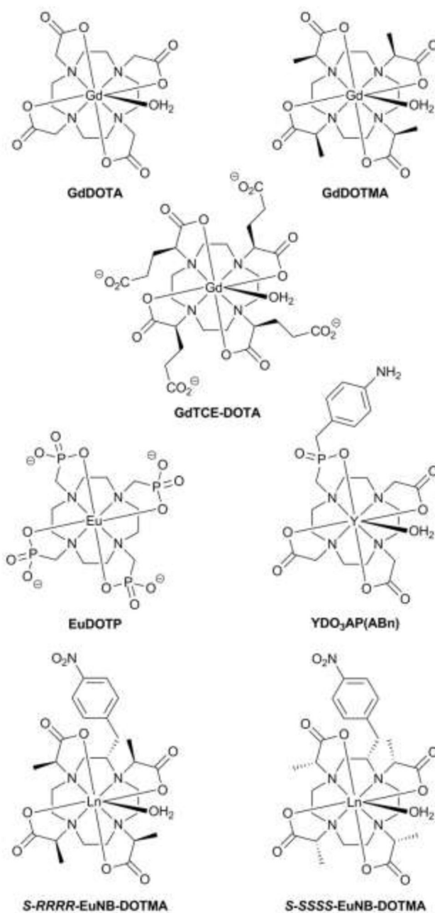
Chart 1. The structures of chelates discussed herein
