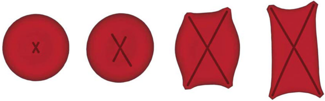
Fig. 3. Successive snapshots of a SS-RBC with the intracellular aligned hemoglobin polymer domain of finite angular width. Two polymer branches are used to represent the angular spanning during the domain development. The final cell morphology resembles a “holly leaf” shape.
