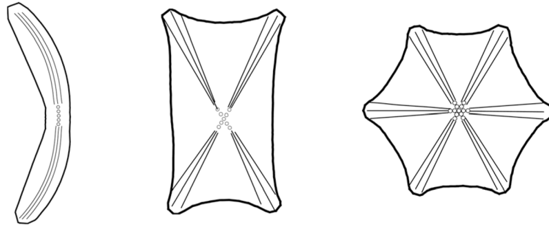
Fig. 1. Sketches of typical cell shapes for deoxygenated SS-RBCs observed in experiments. 9 From left to right, the three sketches represent the “sickle”, “holly leaf” and “granular” shapes of SS-RBCs. The various cell morphologic states are mainly determined by the specific intracellular aligned hemoglobin polymer configurations, represented by the solid lines. The dots represent the post-homogeneous nucleus.
