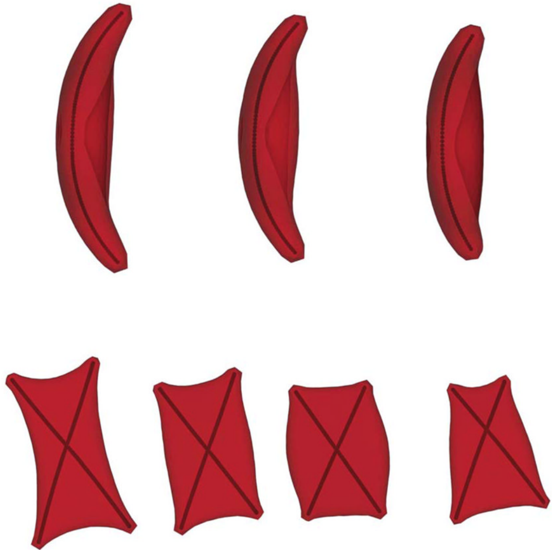
Fig. 5. Final morphologies of the “sickle” (upper) and “holly leaf” (lower) shapes of deoxygenated SS-RBC for different values of cell membrane shear modulus. The “sickle” shape of SS-RBC corresponds to low mean corpuscular hemoglobin concentration value ( 32 \text{ g dL}^{-1} ) and the shear modulus of the cells shown above is set to 20\mu_0 , 40\mu_0 and 70\mu_0 according to experimental measurements. 4 The “holly leaf” shape of SS-RBC corresponds to medium mean corpuscular hemoglobin concentration and the shear modulus is set to 30\mu_0 , 60\mu_0 and 120\mu_0 . We have also included a non-symmetric case in the fourth plot representing a cell morphology with the post-homogeneous nucleus off the cell center with shear modulus 60\mu_0 .
