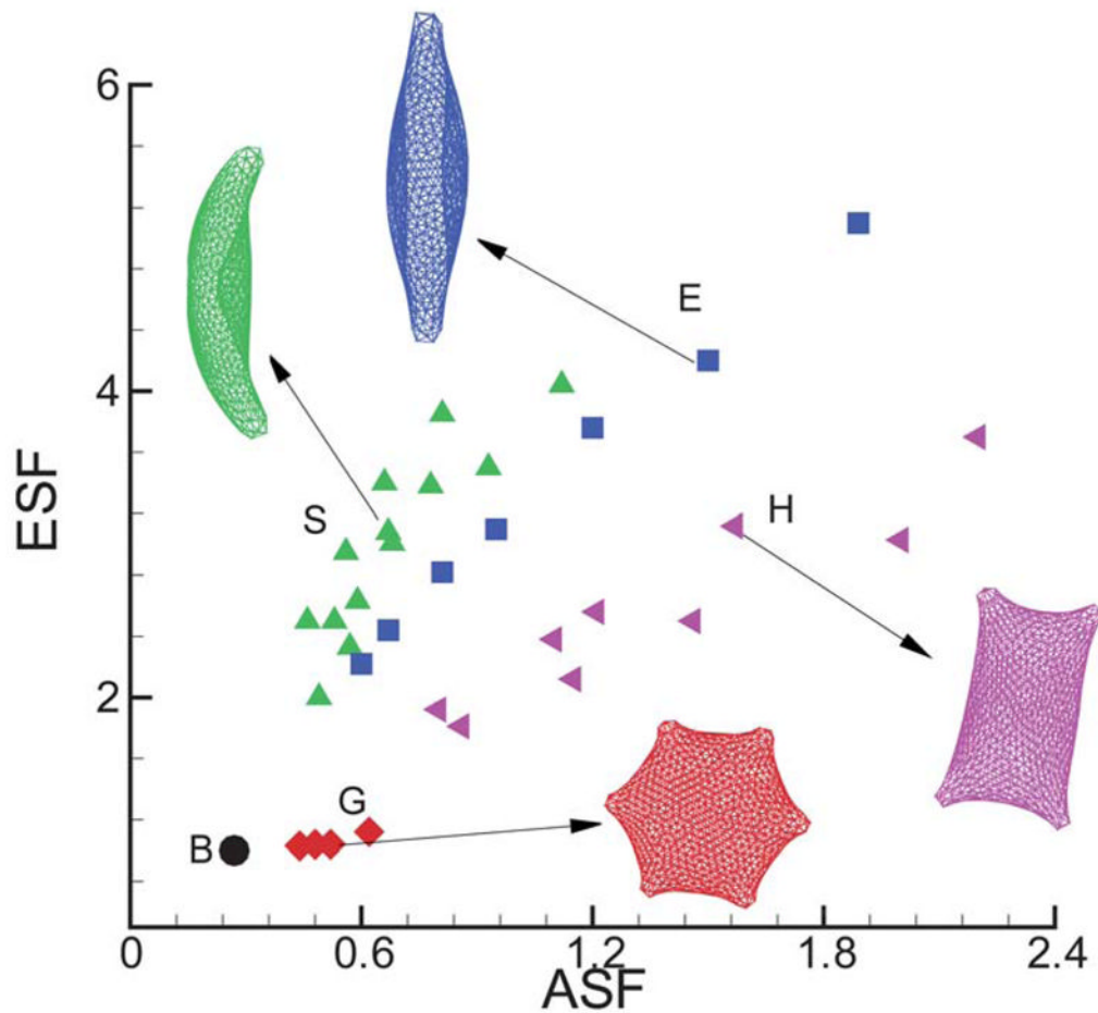
Fig. 7. ASF and ESF for the various cell morphologies obtained. The labels “B”, “G”, “S”, “H” and “E” represent the biconcave, granular, sickle, holly leaf and elongated shapes, respectively. The snapshots show the typical cell shapes for each type of SS-RBC morphology obtained in the present study.
