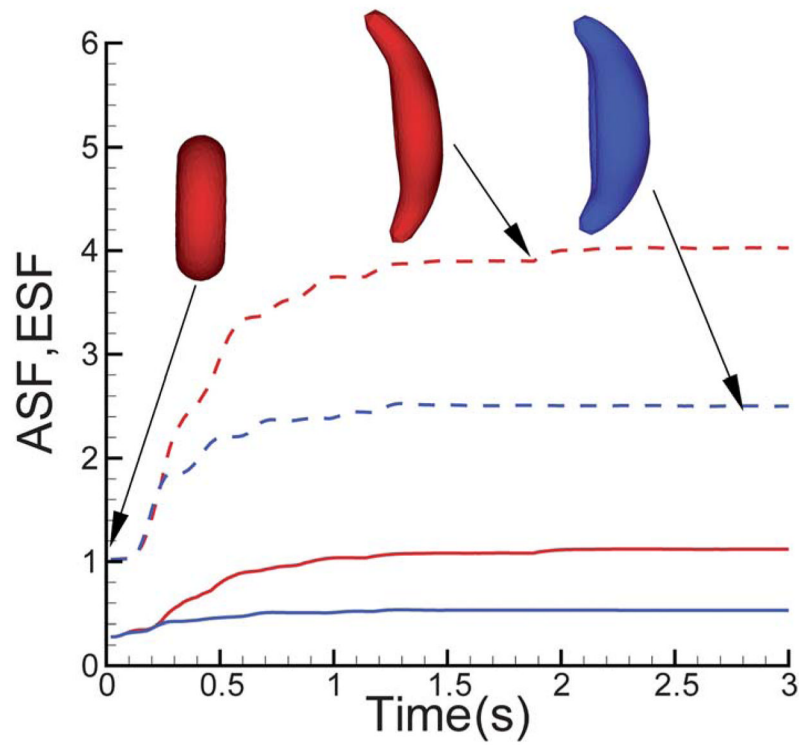
Fig. 6. Instantaneous values of the asphericity (solid lines) and elliptical shape factor (dash lines) of the “sickle” SS-RBC as the aligned hemoglobin polymer domain develops. The red curves correspond to SS-RBC with membrane shear modulus \mu = 30\mu_0 and deflection angle \theta_0 = 179^\circ . The blue curves represent the SS-RBC with shear modulus \mu = 60\mu_0 and \theta_0 = 178.5^\circ .
