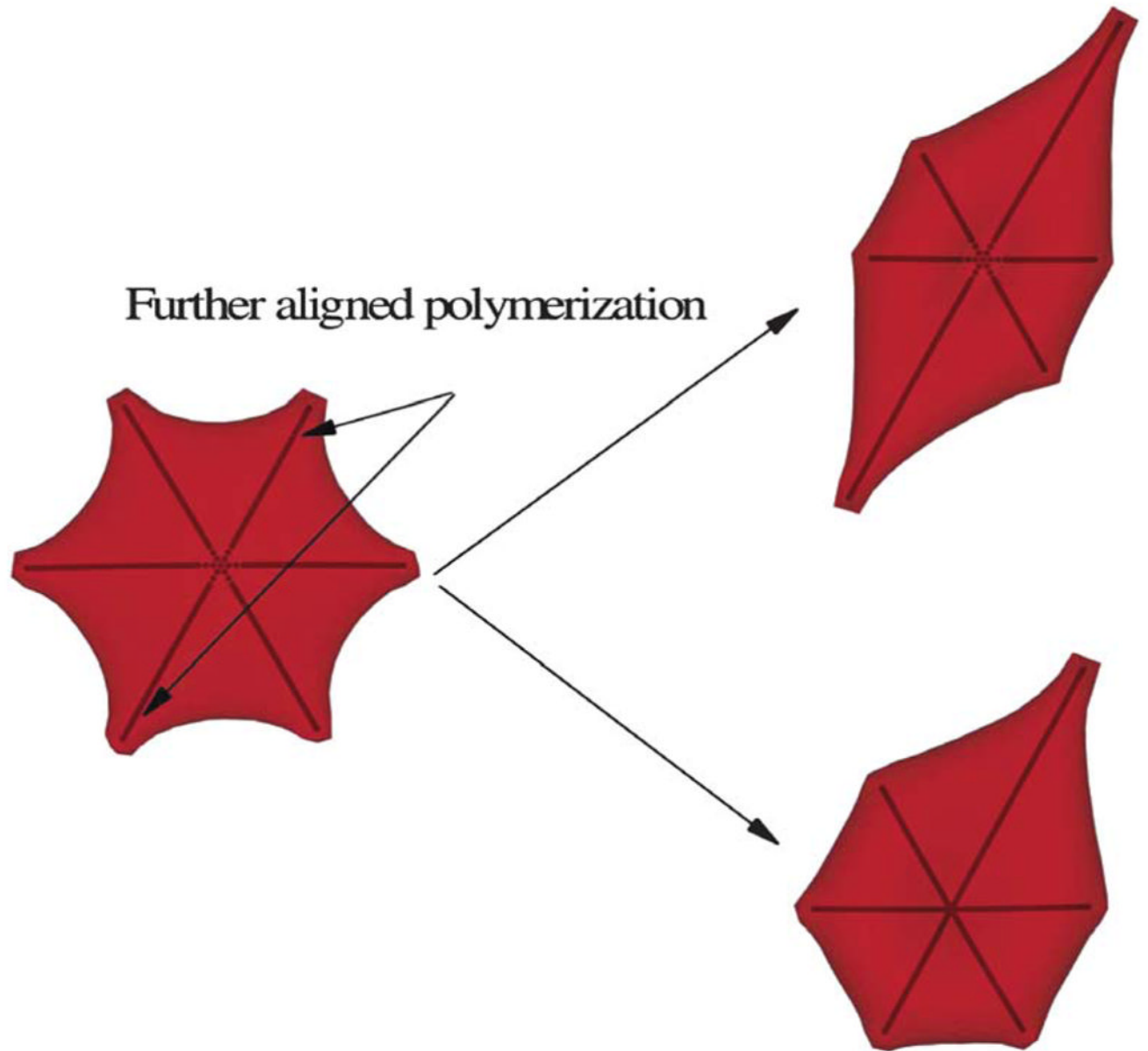
Fig. 9. Elongated shapes: with further aligned polymerization along the specific direction, the granular cell (left) transforms into an “elongated” cell with the cell center keeping the granular shape (upper right), resembling the non-traditional “elongated” cell observed in ref. 9. The lower right plot represents the final cell morphology with the high growth rate imposed only on the upper right direction.
