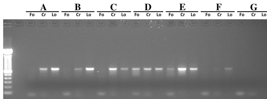
Figure 3 Image of an agarose gel (1.5%) showing PCR products of crustaceans obtained with using different primer pairs. A ), B ) and F ) Pilumnus hirtellus ; C ) and E ) Lophozozymus incisus ; D ) Porcellana platycheles ; G ) Negative control; Fo) LCO1490 and HCO2198 [1]; Cr) CrustDF1 and CrustDR1 (D. Steinke unpublished in [19]); Lo) LoboF1 and LoboR1 (present study).
