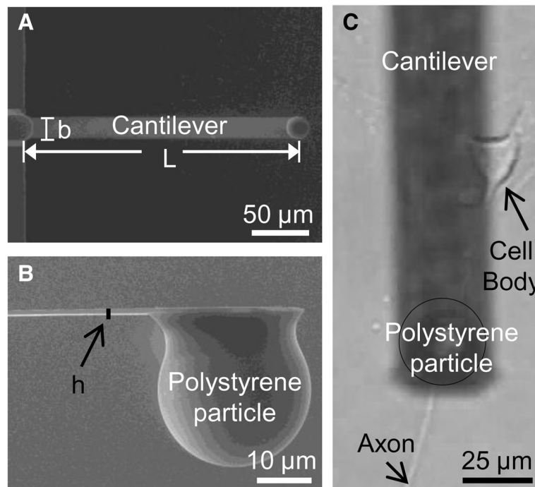
Figure 1 Diagrams illustrating dimension of cantilever and axon being compressed by cantilever in atomic force microscopy (AFM). (A) Top view of a cantilever obtained by scanning electric microscopy (SEM). (B) Side view of a cantilever tip obtained by SEM. (C) Top view of the particle of a cantilever compressing the axon of a dorsal root ganglia (DRG) cell. Image was taken by a digital camera from the eyepiece of the optical part of the AFM.
