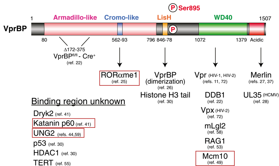
Figure 2 VprBP structural motifs and interacting proteins. The 1507 amino acid human VprBP isoform encoded by transcript variant ENST00000563997 in the Ensembl database (release 71) [29] is shown with the domain features for this isoform as described in the database or in the text. VprBP-interacting proteins are identified below the diagram; those for which the binding site has been mapped are shown below the region mediating the association. Proteins targeted for VprBP-dependent ubiquitination are boxed. The region removed after Cre-mediated deletion of a conditional allele [22], and the location of a DNA-PK-dependent phosphorylation site [30] are also indicated.
