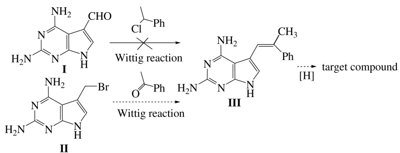
Scheme 1. Attempted synthesis of target compounds.
