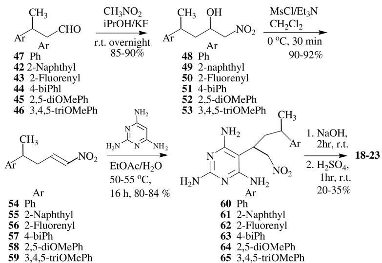
Scheme 4. Synthesis of 18–23 .
