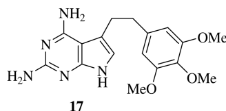
Figure 2. Two atom bridged furo- and pyrrolo[2,3- d ] pyrimidines.
