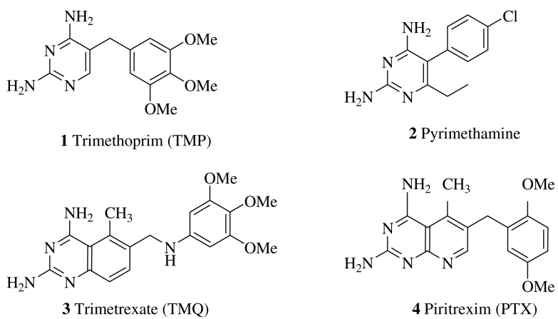
Figure 1. Known inhibitors of pathogenic DHFR.
