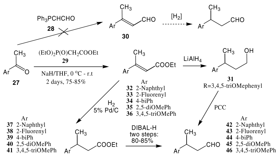
Scheme 3. Synthesis of aldehydes 42–46.
