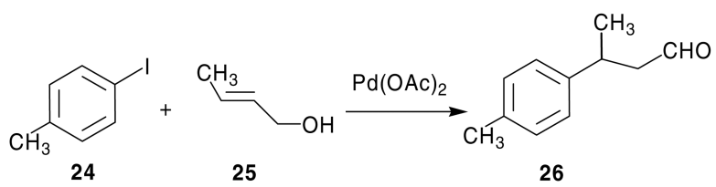
Scheme 2. Heck coupling for the synthesis of 26 .
