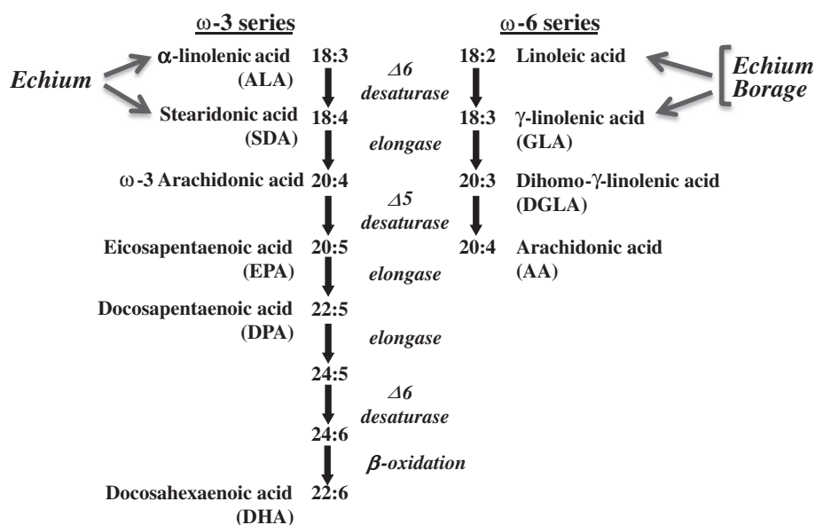
Figure 1 Pathways for metabolism of n-6 (left) and n-3 (right) PUFAs in humans. The pathway depicts the synthesis of 20 and 22 carbon PUFAs from the essential, dietary PUFAs, α-linolenic acid (n-3) and linoleic acid (n-6). The PUFAs derived from borage oil (linoleic and gamma-linolenic acids, both n-6) and echium (α-linolenic, n-3; stearidonic, n-3; linoleic and gamma-linolenic acids, both n-6) would be expected to enter the pathways at the indicated points.
