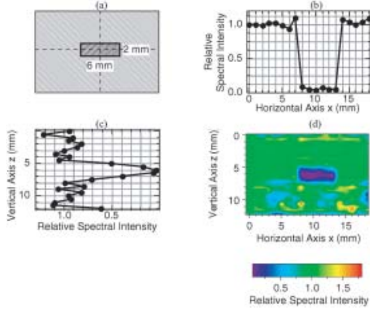
Fig. 3. a. Cross-sectional view of the object buried in a scattering medium. b. One-dimensional (1D) image of the scattering medium horizontally across the center of the object as indicated by the horizontal dashed line in panel a. c. 1D image of the scattering medium vertically across the center of the object as indicated by the vertical dashed line in panel a. d. Two-dimensional tomographic image of the object buried in a scattering medium.
