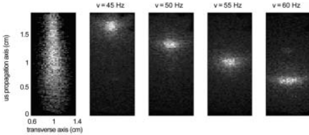
Fig. 6. Demonstration of the virtual source of ultrasound-modulated light. Left frame: the entire virtual source. Following frames: virtual sources corresponding to various values of \nu obtained by adjusting the frequency f_h .
