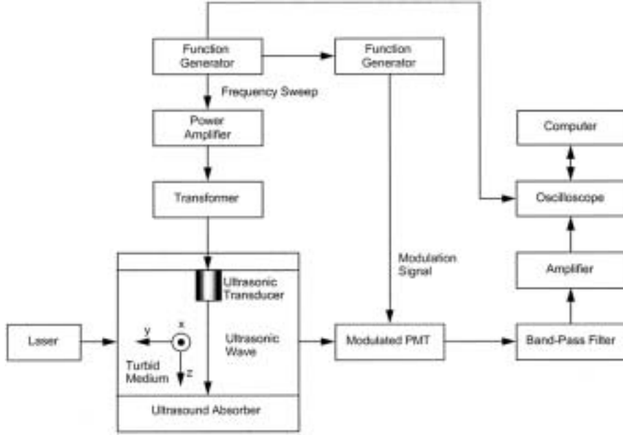
Fig. 1. Schematic of the experimental setup for Fourier-transform acousto-optic tomography (AOT).
