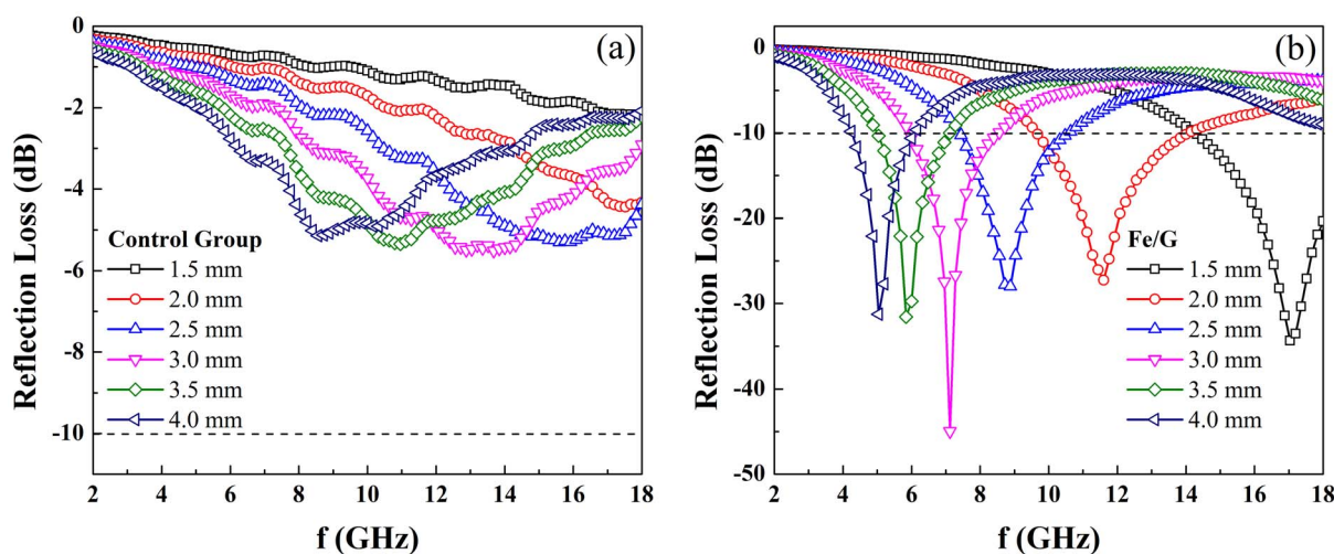
Figure 6 | Calculated reflection loss of different thickness for (a) control group, and (b) Fe/G. The dash line is a guide of eye to show the frequency range in which RL is less than -10 \text{ dB} .
