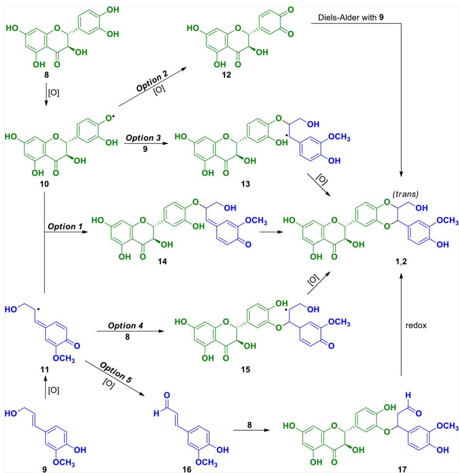
Scheme 1. Mechanistic Options for the Biomimetic Synthesis of Flavonolignans
