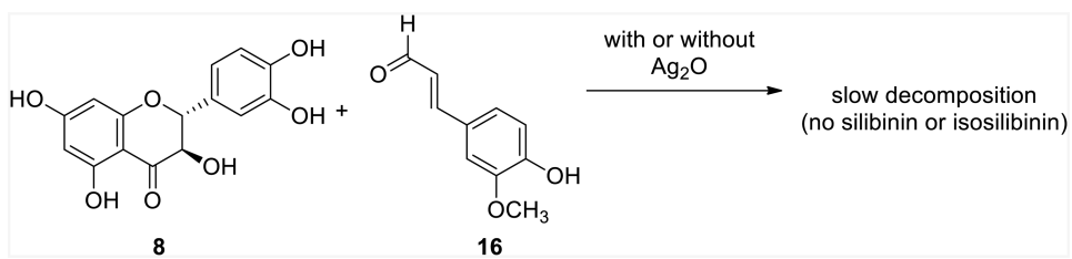
Scheme 5. Attempted Coupling of Coniferyl Aldehyde to Taxifolin
