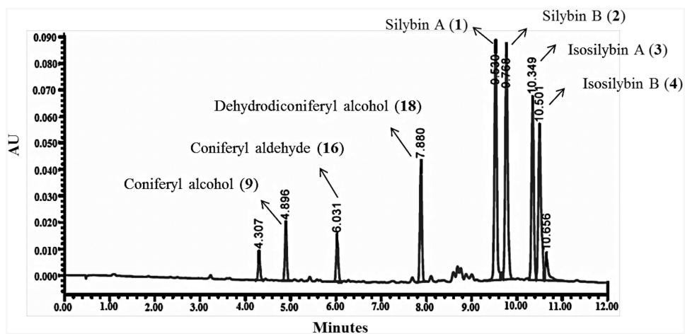
Figure 2. UPLC chromatogram of biomimetic reaction using conditions in Scheme 2. UPLC was conducted using a CH 3 OH/H 2 O (0.1% formic acid) gradient that initiated at 5:95 and increased to 50:50 over 10 min and held at that ratio for 2 min at a flow rate of 0.6 mL/min (50°C) using an HSST3 column monitored at 288 nm.
