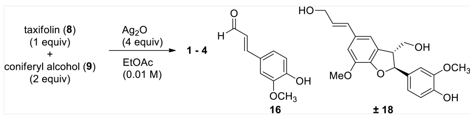
Scheme 2. Biomimetic Synthesis of Silibinin, Isosilibinin, and Other Byproducts
