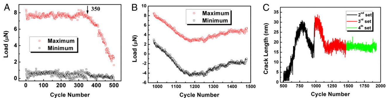
Fig. 3. Maximum/minimum loads under a fixed value of imposed displacement amplitude and crack length evolution as a function of fatigue cycles. (A) Load vs. cycle number for the first set of tests spanning 490 cycles. (B) Load vs. cycle number for the third set from 981 to 1,470 cycles. (C) Crack length evolution with increasing cycle number.
