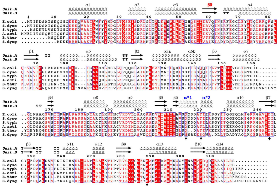
Figure 2. Sequence alignment of various LsrR proteins
