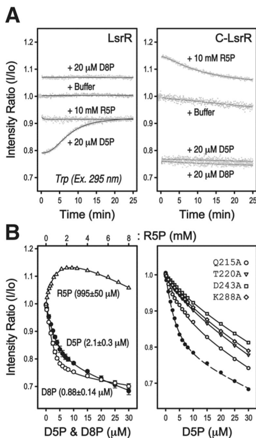
Figure 4. The ligand-binding of the LsrR proteins was monitored by using the intrinsic Tyr/Trp fluorescence
