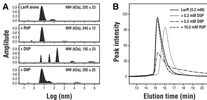
Figure 6. The molecular sizes of the LsrR protein in the absence and the presence of ligand molecules.
