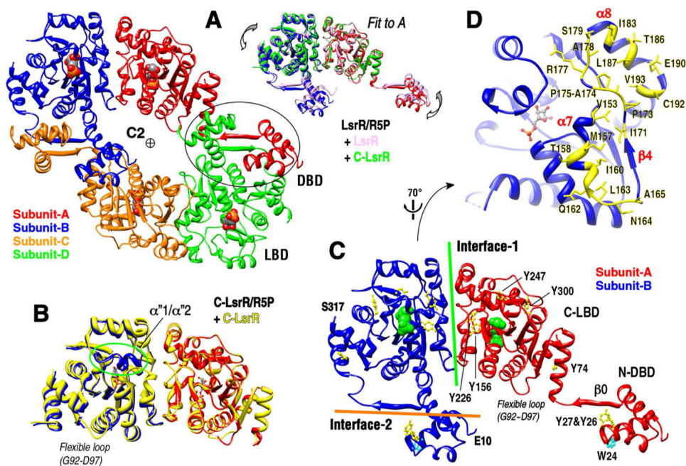
Figure 1. Structural overviews of the LsrR tetramer and the C-LsrR dimer
