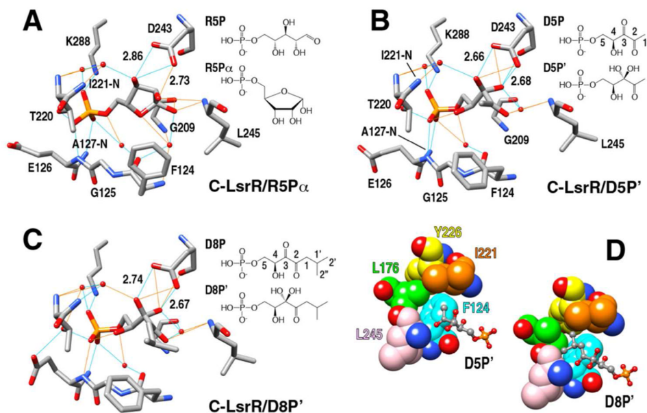
Figure 3. Ligand recognitions of LsrR for three different ligand molecules
