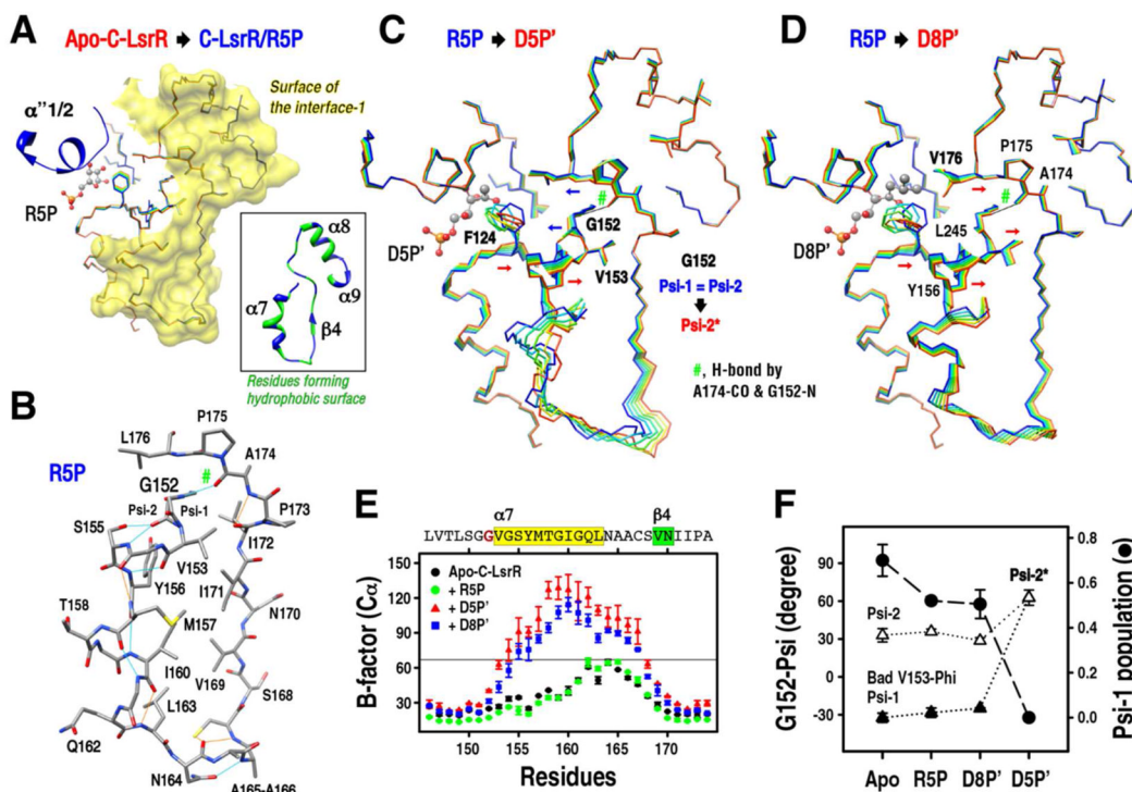
Figure 5. The dimeric interface-1 was disrupted by the binding of D5P', but not by that of R5P and D8P'
