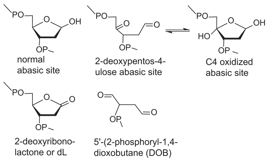
Figure 5. Structure of the main oxidized a basic sites identified in isolated DNA (C4-AP in equilibrium with the acyclic 2-deoxypentose-4-ulose abasic site, DOB, 2-deoxyribonolactone or dL).
