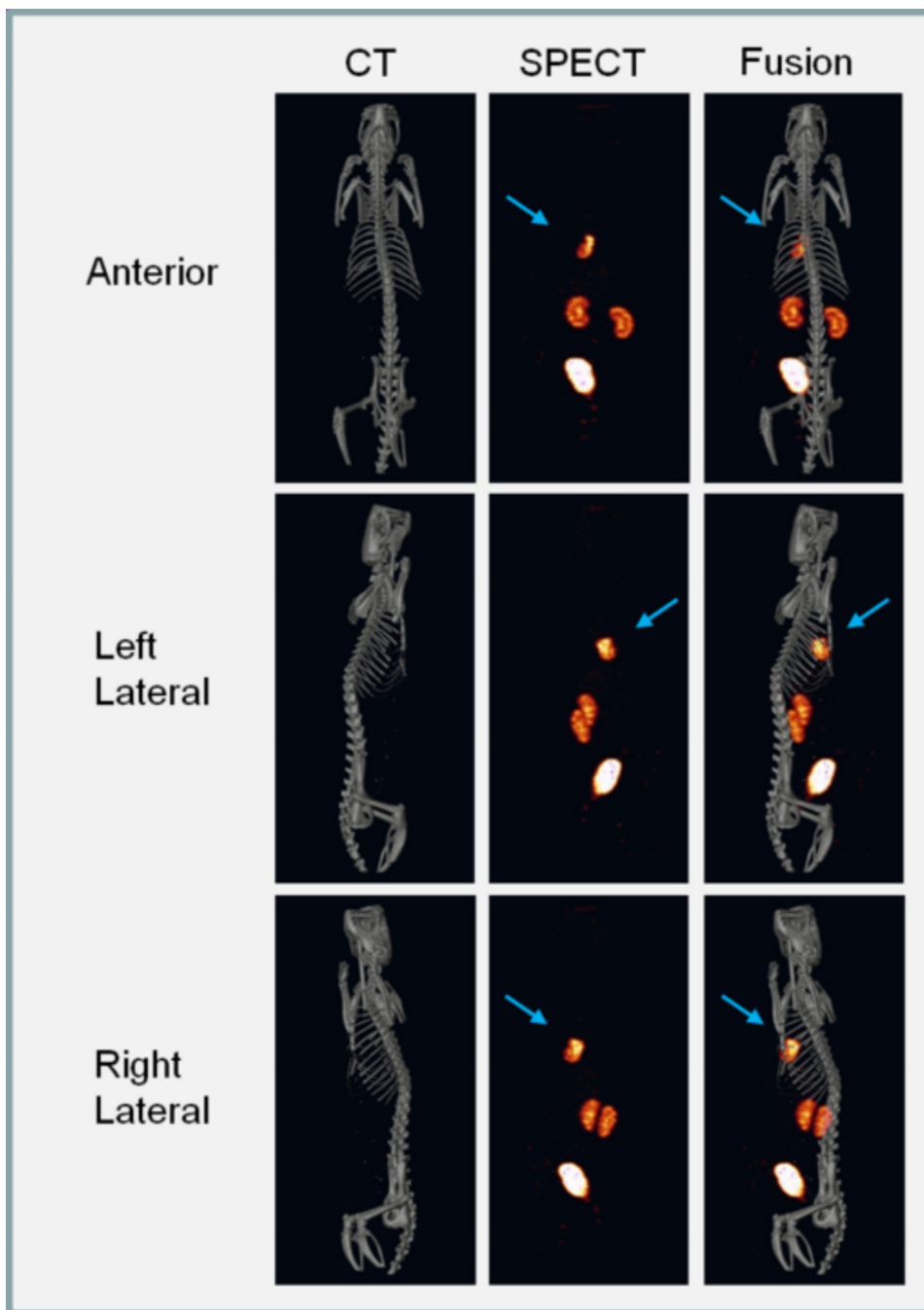
Figure 2. Representative SPECT/CT images of ^{99m}\text{Tc} -Duramycin uptake in ischemically damaged cardiac tissue in vivo. The CT, SPECT and SPECT/CT fusion images are shown in the left, middle and right columns, respectively. Radioactivity uptake in the left ventricular free wall is highlighted with an arrow in the tomographic images.
