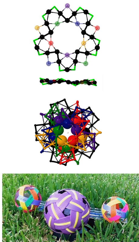
Figure 4. Selected Characteristics of I-Au_{144}Cl_{60}^{[2+]} . ( Top ) A single strand (black) is identified by continuation of the radial elements identified in Fig. 3 (right). The black circles and green elbows constitute a single closed loop. Thick connecting lines designate the short bonds; the five (5) sets of distinctly coloured spheres mark under- and over-crossings of the other five strands. In side-view , the structure is essentially flat, incorporating the two coplanar regular decagons from the 30- Au shells (Fig. 1, in orange), the nearly 10 nearly coplanar sites from the 60- Au shell (blue in Fig. 1), and the zig-zag pattern of the 60- X sites (10 lime-green elbows) ( Centre ) Hemisphere view of all six (6) coloured strands, obtained by elaboration from the single strand. All but 24 sites (the two 12- Au shells) of the 204 sites are incorporated into the weave structure. ( Bottom ) Photograph of a standard woven kickball ( Sepak Tetraw in the Thai language) on Texas Grass. It displays the same 6-strand network topology, including chirality, as that identified herein for the I-Au_{144}X_{60} structure, thus serving an aide memorandum to the entire structure.
