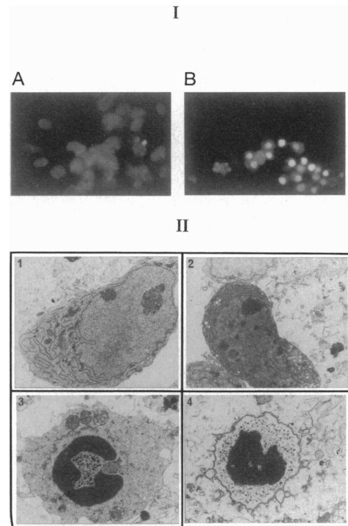
FIG. 2. Documentation of KA-mediated apoptosis of cultured neurons. (I) In situ DNA fragmentation assay using terminal transferase mediated dUTP nick-end labeling (TUNEL) method. Spinal cord neurons untreated (A) or treated with 0.1 mM KA (B). Fluorescence signals were obtained by excitation of fluorescein isothiocyanate at 485 nm. (II) Transmission electron micrographs showing typical stages of neurons undergoing KA-mediated apoptosis. (1) Untreated neuron. (2) Neuron at early stages of apoptosis. (3 and 4) Advanced apoptosis: patches of condensed chromatin and abundant vacuoles. ( \times 56,700 .)
