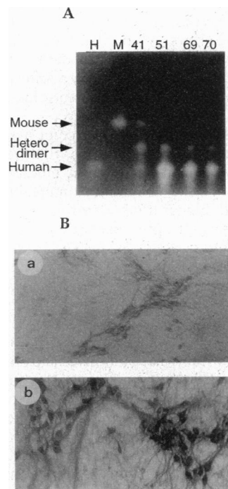
FIG. 1. (A) Polyacrylamide gel analysis of Cu/Zn SOD enzymatic activity in brain extracts from control and different lines of Tg-Cu/Zn SOD mice. The positions at which the active human (H) and mouse (M) Cu/Zn SOD enzymes migrate are indicated. (B) Immunostaining of cultured neurons with anti-human Cu/Zn SOD antibodies. (a) Nontransgenic. (b) Cultures derived from TgHS-51 embryos. ( \times 140 )
