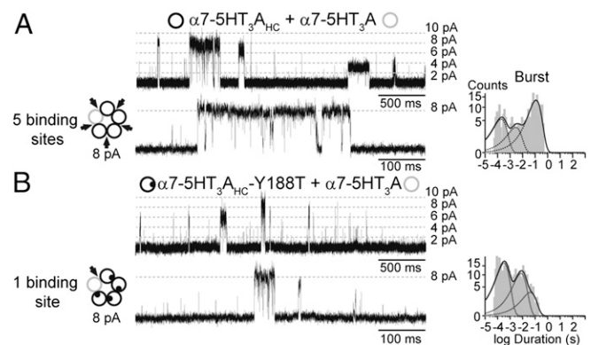
Fig. 5. Duration of bursts of \alpha 7 -5HT 3 A containing five or one functional binding sites. Cells were cotransfected with control ( \alpha 7 -5HT 3 A) and high-conductance ( \alpha 7 -5HT 3 A Hc ) subunits carrying (B) or not (A) Y188T mutation. Single channels were recorded in the presence of 1 mM ACh and 2 mM 5-HI at -120 mV. Channels of the amplitude class determined by four high-conductance subunits were analyzed, which correspond to arrangements containing five (A) or one (B) functional binding sites.
