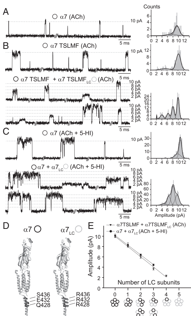
Fig. 3. Electrical fingerprinting for \alpha 7 . (A) Single-channel currents activated by 100 \mu M ACh from wild-type \alpha 7 . Amplitude histogram constructed with events longer than 0.3 ms. (B) Single-channel currents activated by 100 \mu M ACh from cells transfected with \alpha 7TSLMF alone (Upper) or together with \alpha 7TSLMF_{LC} (Lower) (subunit ratio 1:1). (C) Single-channel currents activated by 100 \mu M ACh in the presence of 2 mM 5-HI from cells transfected with \alpha 7 alone (Upper) or together with \alpha 7_{LC} (Lower) (subunit ratio 1:1). The two traces for the mixed subunits are excerpts from the same recording. Representative amplitude histograms are shown. Membrane potential: -70 mV. (D) Homology model of a single \alpha 7 subunit based on the Torpedo AChR structure (PDB ID code 2BG9), with the mutations that lead to the low-conductance form of \alpha 7 ( \alpha 7_{LC} ). (E) Plot of mean current amplitude against number of mutant low-conductance subunits. The fitted slopes are: 1.89 pA/LC subunit for \alpha 7 + \alpha 7_{LC} in the presence of ACh + 5-HI and 1.97 pA/LC subunit for \alpha 7TSLMF + \alpha 7TSLMF_{LC} in the presence of ACh. Note that \alpha 7 wild-type conductance is referred to as high conductance.
