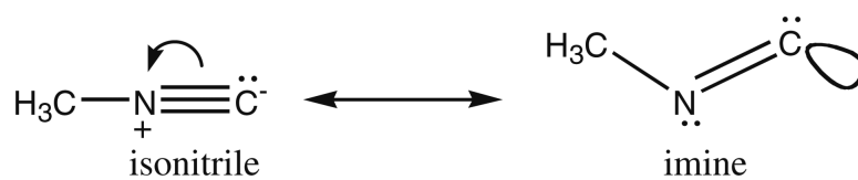
Scheme 1. Resonance structures for methyl isocyanide
