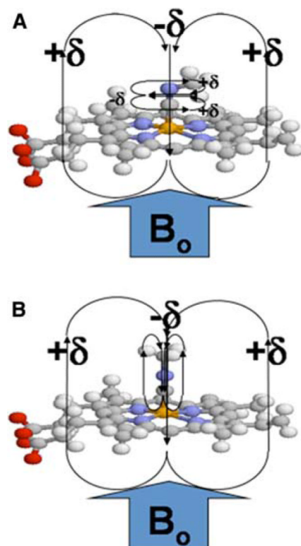
Fig. 1. Methyl isocyanide bound to the heme iron. Schematic representation of methyl isocyanide bound to heme with (a) an iron-carbon bond order of two (“bent”) and (b) an iron-carbon bond order of one (“linear”). The heme pyrrole rings, along with the CN triple (or double) bond, produce a highly anisotropic environment that can produce large chemical shift perturbations for the labeled methyl group
