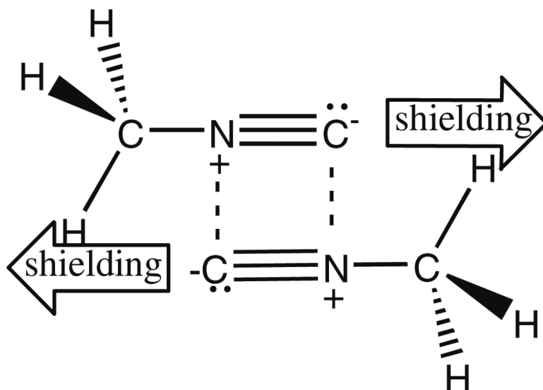
Scheme 2. Proposed methyl isocyanide dimer in nonpolar solvent
