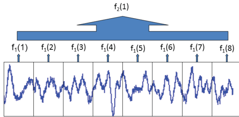
Figure 1. Pictorial Description of hierarchical feature computation.
