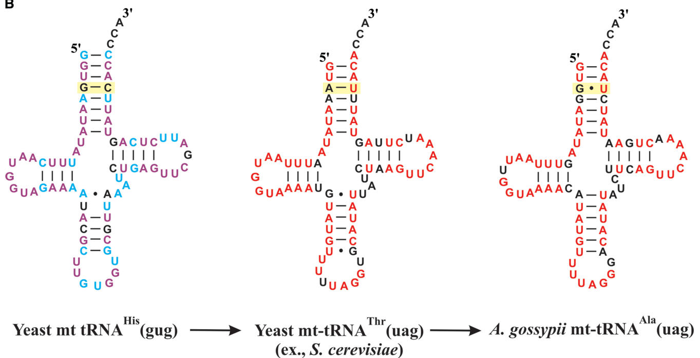
Figure 2. Primary and secondary structures of yeast mitochondrial tRNA Ala UAG , tRNA Thr UA G and tRNA His GUG . (A) Selected yeast mitochondrial tRNAs with UAG or GUG anticodons (anticodon marked orange) are aligned (upper and lower blocks of sequences, respectively). Square brackets indicate the four standard helical regions in tRNAs. The arrow points to a nucleotide insertion that leads to a characteristic 8-nt anticodon loop in tRNA Thr UA G (tRNA Thr UA G). In A. gossypii , the anticodon loop has 7 nucleotides, and this tRNA reads CUN codons as Ala but not Thr. As tRNA Thr UA G is most likely derived from tRNA His by duplication, tRNA His is included in the alignment for comparison [see also (21)]. Note the characteristic G residue at position -1 (constituting the 5'-terminus of tRNA His ) that pairs with the C at the 3'-discriminator position (both positions marked in gray). (B) Secondary structures of tRNAs that illustrate a possible tRNA reassignment scenario, S. cerevisiae tRNA His GUG (left), A. gossypii tRNA Ala UAG (right) and S. cerevisiae tRNA Thr UA G (middle). Nucleotide identity is coded as follows; red, A. gossypii tRNA Ala UAG versus S. cerevisiae tRNA Thr UA G; magenta, identity across all three tRNAs; and blue, additional identity between A. gossypii and S. cerevisiae tRNA His GUG . Following a codon capture mechanism, tRNA Ala UAG and tRNA Thr UA G would have evolved from a tRNA Ala UAG because the latter is present in the sister lineage Lachancea species (for a species phylogeny, see Figure 5), and absent in K. lactis . For abbreviations, see Figure 1.
