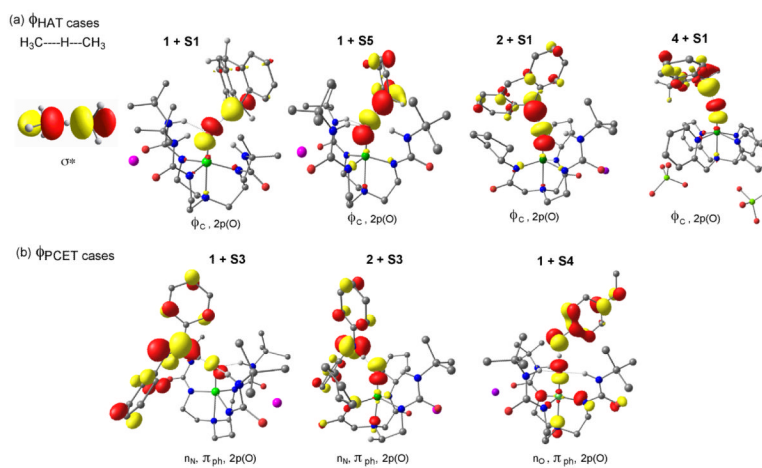
Figure 8. SNOs in TSs: (a) \phi_{\text{HAT}} type SNOs for 1+S1 , 1+S5 , 2+S1 , and 4+S1 , shown alongside the \phi_{\text{HAT}} orbital in the TS ( \text{H}_3\text{C}\cdots\text{H}\cdots\text{CH}_3 ). (b) \phi_{\text{PCET}} type SNOs for 1+S3 , 2+S3 , and 1+S4 . The hydrogen atoms not in \text{O}\cdots\text{H}\cdots\text{X} moiety are omitted for clarity.
