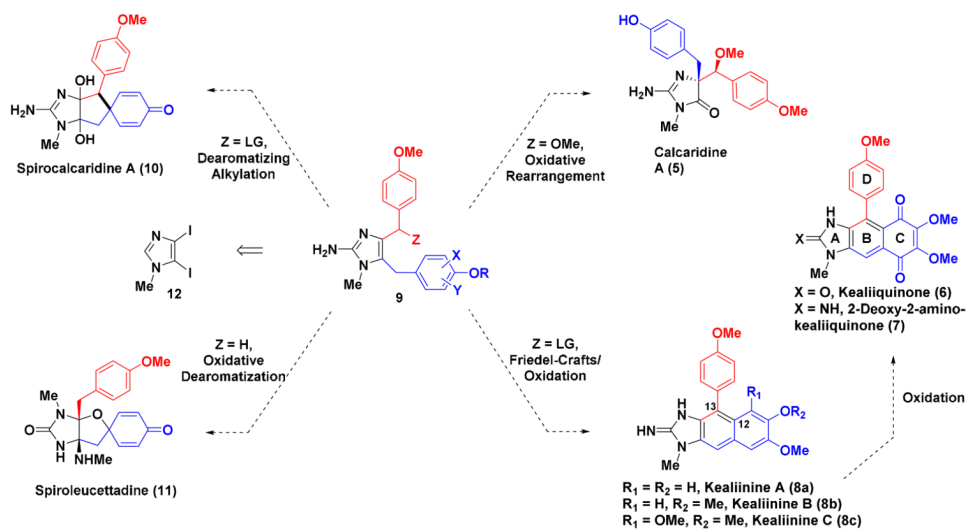
Figure 2. Putative biosynthetic relationships among the Leucetta alkaloids
