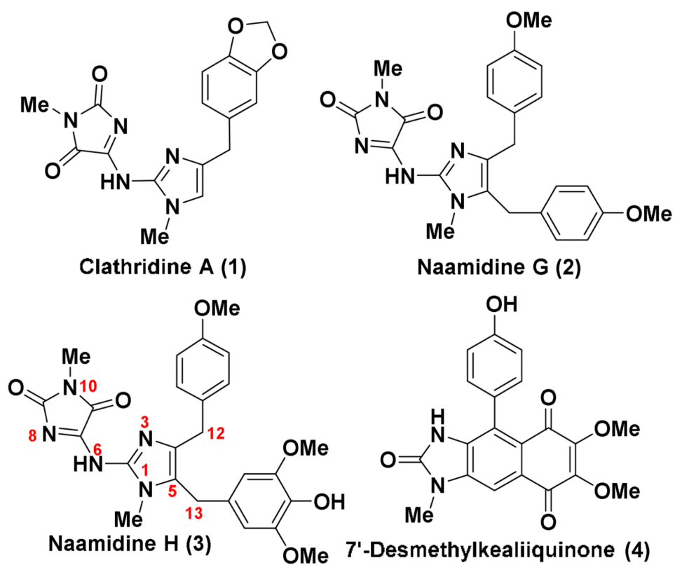
Figure 1. Structures of the Leucetta -family of alkaloids
