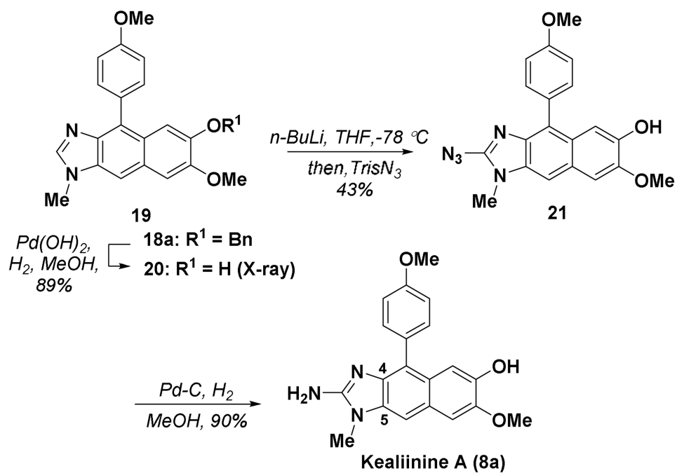
Scheme 2. Completion of kealiinine A ( 8a ).
