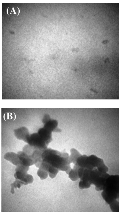
Fig. 6. Characterization of AgNP. A drop of the original solution was placed on a carbon-coated copper grid, air dried, and observed with ZIESS electron microscope (EM902A) at 80KV. Pictures (A) spherical around 10 nm, and (B) agglomerated structures above 150, were taken from different areas of one single grid. Most of the grid was covered with agglomerations. (Scale markers indicate 50 nm ( \times 140000 ) and 150 nm ( \times 50000 ), respectively).
