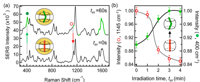
Figure 3. (a) SERS spectra of DAS \subset CB[7]:AuNP nanocluster solution before ( t_{\text{irr}} = 0 s, trans -) and after ( t_{\text{irr}} = 60 s, cis -) UV irradiation ( \lambda = 355 nm). Highlighted modes (green, t_{\text{irr}} = 60 s) indicate significant amplitude changes following photoisomerization. Complexed DAS concentration 1 nM. Spectra offset and background subtracted for clarity. (b) Time-resolved normalized SERS intensity of characteristic modes for the reactant trans -DAS ( \circ ) and product cis -DAS ( \bullet ) identified in (a) following subsequent photoirradiation. Solid and dashed lines guide the eye.
