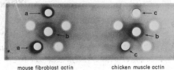
FIG. 2. Immunodiffusion of actin antiserum. (a) 4 \mu\text{g} (upper hole) and 2 \mu\text{g} (lower hole) of a 30% ammonium sulfate cut from mouse fibroblasts. The heavy precipitate around the holes is due to aggregated actin. (b) 20 \mu\text{l} of partially purified rabbit antiserum. (c) 5 \mu\text{g} (upper) and 2 \mu\text{g} (lower) of purified chicken muscle actin. Immunodiffusion was performed at 37^\circ for 24 hr. The plates were washed for 24–36 hr at room temperature in 0.15 M NaCl, 0.01 M Tris·HCl (pH 7.5). They were subsequently stained in 0.25% Coomassie brilliant blue–50% methanol–7.5% acetic acid for 1 hr, destained in 7.5% methanol–7.5% acetic acid, and photographed.
