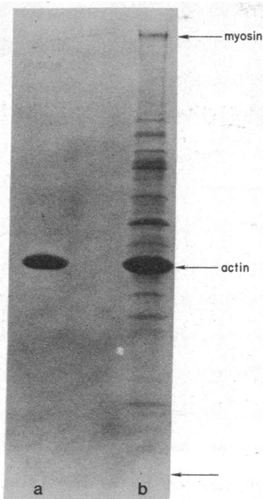
FIG. 1. SDS gel electrophoresis of actin. SDS polyacrylamide slab gel electrophoresis was performed in 12.5% slabs according to Studier (19). (a) Highly purified chicken muscle actin (10 \mu\text{g} ). (b) A 30% ammonium sulfate cut of a low-salt extract from an ethanol powder of mouse fibroblasts (15 \mu\text{g} ). A small amount of myosin copurifies with actin under the extraction conditions used (see Materials and Methods ). The arrow at the bottom of the figure shows the dye front of the gel.
