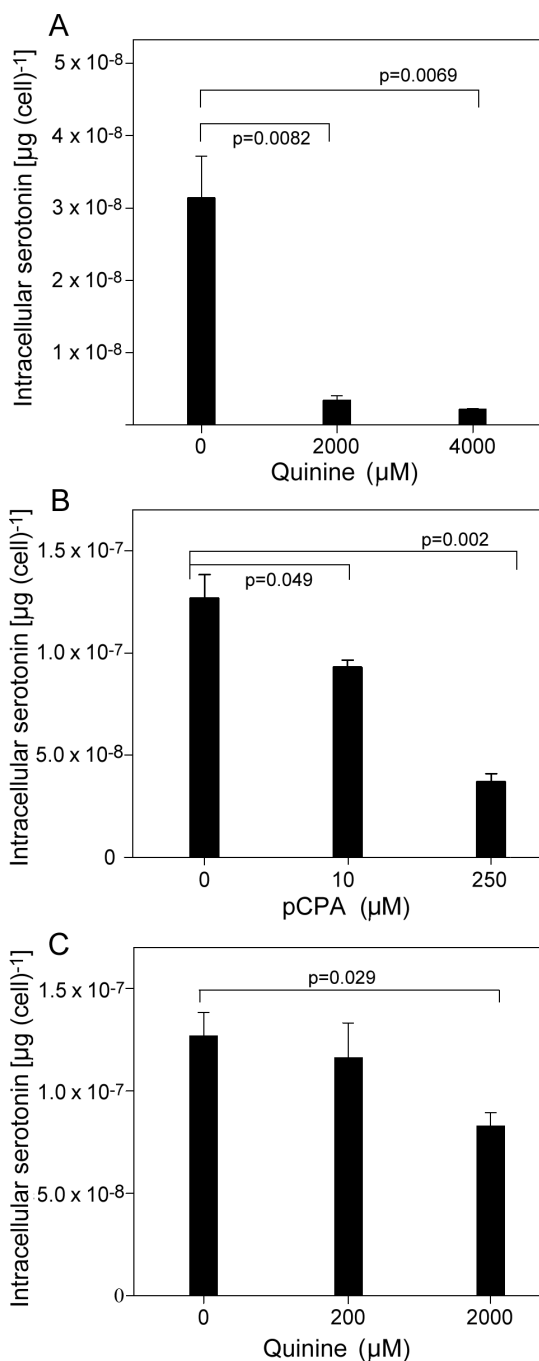
Figure 4 | Quinine inhibits serotonin production. (A) Yeast cells transformed with pYES-TDC were cultured for 24 h in the presence of the indicated quinine concentration before determination of cellular serotonin with HPLC-ED. (B) Serotonin was determined in rat RN46A cells after 5 d culturing with the indicated concentration of the TPH2 inhibitor, pCPA. (C) Serotonin was determined in rat RN46A cells after 5 d culturing with the indicated concentration of quinine. Mean values are shown \pm SEM from three independent experiments.
