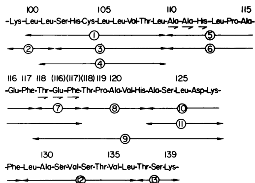
FIG. 3. The proposed sequence of the core section of the \alpha chain of Hb-Grady. Numbers above residues refer to positions in chains, and the numbers in circles to the fragments listed in Table 2.
