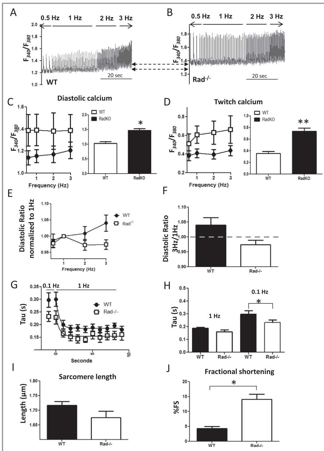
Figure 5. Diastolic calcium is elevated, dynamic range of frequency response is absent, and sarcomeric shortening is increased in Rad -/- cardiomyocytes. A and B, Representative F 340/380 traces in isolated adult cardiomyocytes at multiple pacing frequencies. C and D, F 340/380 ratios of wild-type (WT) and Rad -/- ventricular myocytes at diastole (C) and peak height (D). Bar graph: data averaged at 1 Hz. n=27 cells (5 mice) for WT, n=42 cells (8 mice) for Rad -/- . E and F, Diastolic F 340/380 normalized to 1 Hz (E). 3 Hz to 1 Hz is shown as a measure of diastolic dynamic range (F). n=16 cells (3 mice) for WT, n=13 cells (4 mice) for Rad -/- . G, Calcium transient decay rate ( \tau ) of Rad -/- and WT as pacing is increased from 0.1 Hz to 1 Hz. n=8 cells (3 mice) for WT, n=12 cells (3 mice) for Rad -/- . H, The change in \tau is significantly different between Rad -/- and WT at 0.1 Hz. n=8 cells (3 mice) for WT, n=12 cells (3 mice) for Rad -/- . I, Diastolic sarcomere length trends towards shorter in Rad -/- . J, Fractional shortening (FS) in WT and Rad -/- ventricular myocytes paced at 0.1 Hz. n=16 cells (3 mice) each for WT and Rad -/- . * P <0.05, ** P <0.01, *** P <0.001 vs WT. Error bars represent SEM.
