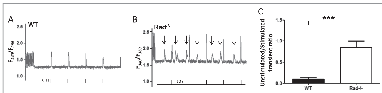
Figure 7. \text{Rad}^{-/-} calcium transients display spontaneous activation at low frequency. A, Representative wild-type (WT) calcium transients showing initial 3-Hz stimulation followed by 0.1 Hz. B, Spontaneous cytosolic calcium transients spontaneously occur in isolated adult ventricular myocytes from \text{Rad}^{-/-} mice paced at 0.1 Hz. Arrows indicate spontaneous transients. Solid lines with vertical tick marks indicate stimuli once every 10 s. C, Quantification of spontaneous transients in \text{Rad}^{-/-} and WT cohorts. n=37 cells (5 mice) for WT, 36 cells (8 mice) for \text{Rad}^{-/-} . *** P<0.001 vs WT. Error bars represent SEM.
