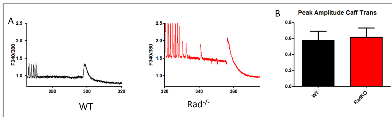
Figure 6. SR \text{Ca}^{2+} load measured as caffeine-releasable \text{Ca}^{2+} is not different between \text{Rad}^{-/-} and wild-type. A, Representative traces. B, Pooled peak amplitude of caffeine induced \text{Ca}^{2+} release. SR indicates sarcoplasmic reticulum.
