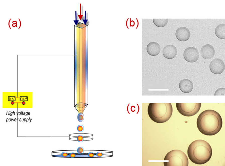
FIG. 4. (a) Schematic of the formation of aqueous droplets in the all-aqueous electrospay approach; (b) optical microscopic images of monodisperse aqueous droplets produced by all-aqueous electrospay; (c) microscopic images of all-aqueous emulsions with a core-shell structure; droplets are collected on a glass slide. Scale bar is 200\ \mu\text{m} .
