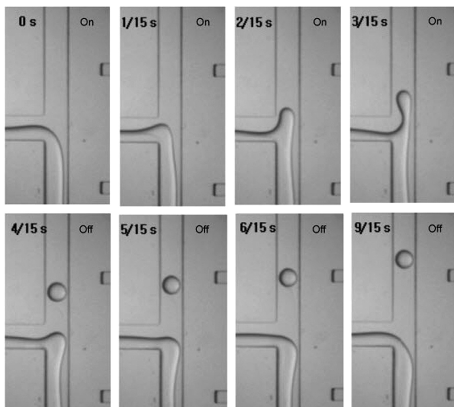
FIG. 3. Formation of a w/w emulsion induced by electro-hydrodynamic chopping. The width of channel is 200\ \mu\text{m} . Reprinted with permission from Song et al. , J. Chromatogr. A 1162 , 180 (2007). Copyright 2007 Elsevier.
