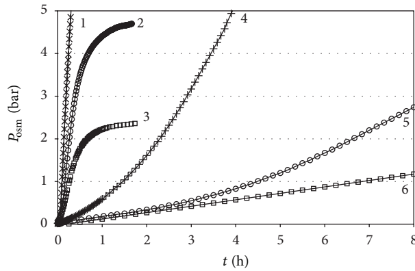
FIGURE 4: Osmotic pressure P_{osm} versus time t dependence for three different initial sucrose concentrations at the two regimes: (1) 0.5 M (constant volume); (2) 0.2 M (constant volume); (3) 0.1 M (constant volume); (4) 0.5 M (variable volume); (5) 0.2 M (variable volume); (6) 0.1 M (variable volume).
