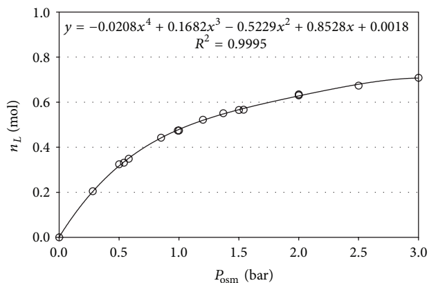
FIGURE 2: Solvent influx n_L [mol] as a function of osmotic pressure P_{osm} [bar] in the regime of variable solution volume.
