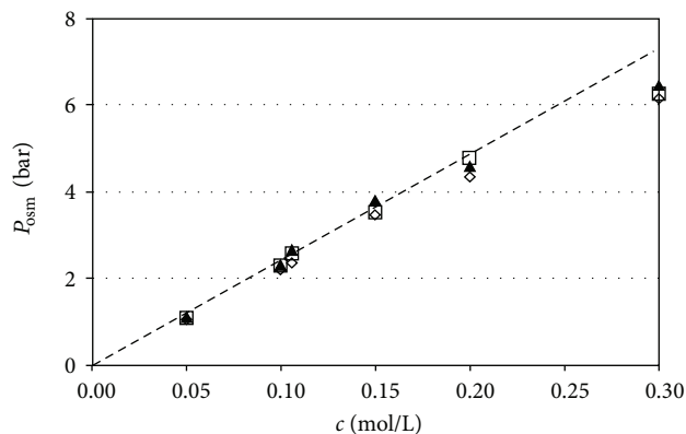
FIGURE 3: Comparison of equilibrium osmotic pressure values, P_{osm} as a function of solute concentration under regimes of constant and variable solution volume. Experimental data are from the readings of the electronic pressure sensor, respectively: ( \square ) constant solution volume; ( \diamond ) variable solution volume; ( \blacktriangle ) variable solution volume (values corrected for dilution). The dotted line indicates the theoretical dependence (see (1)).
