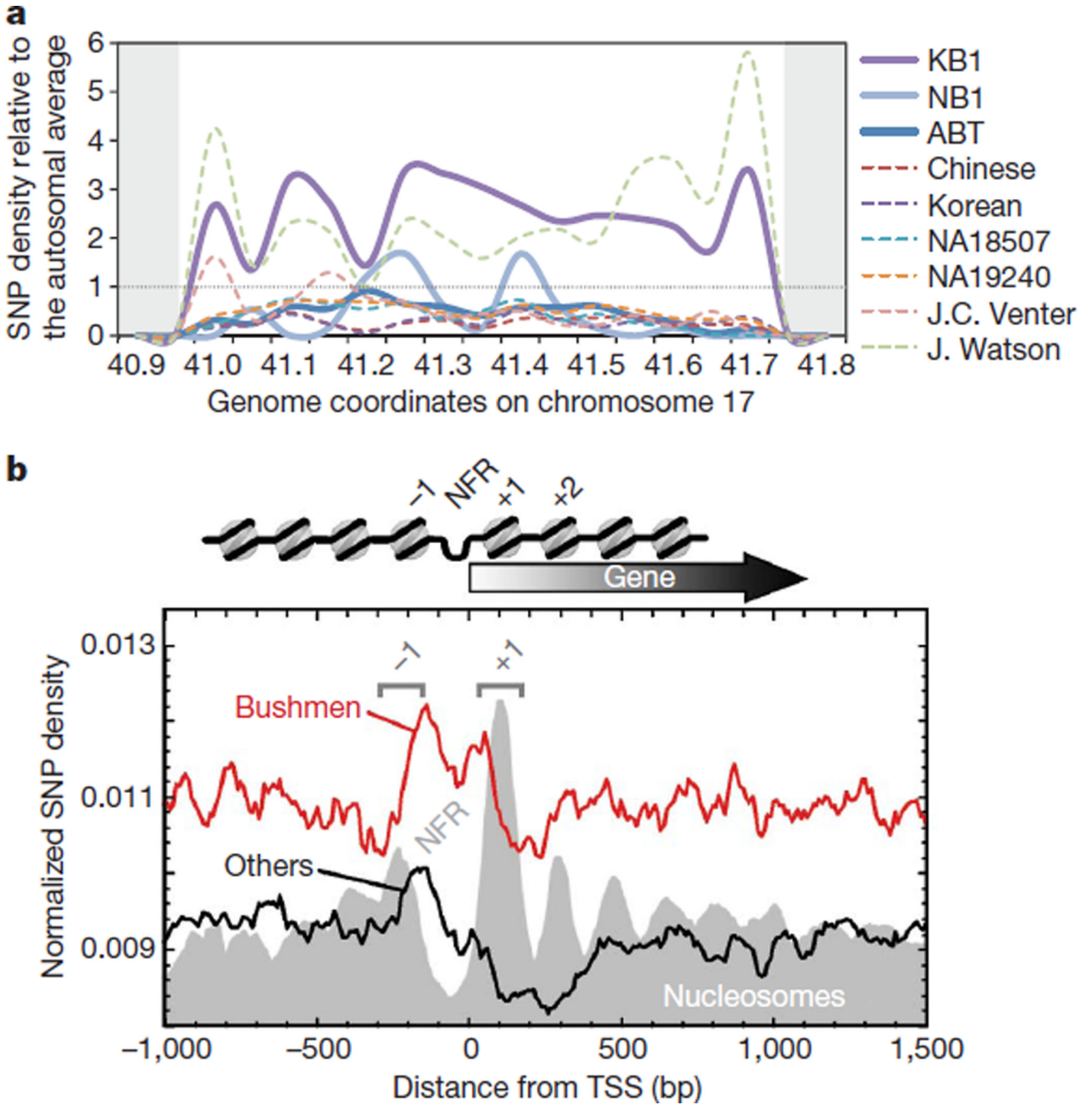
Figure 3. Variation in SNP densities
