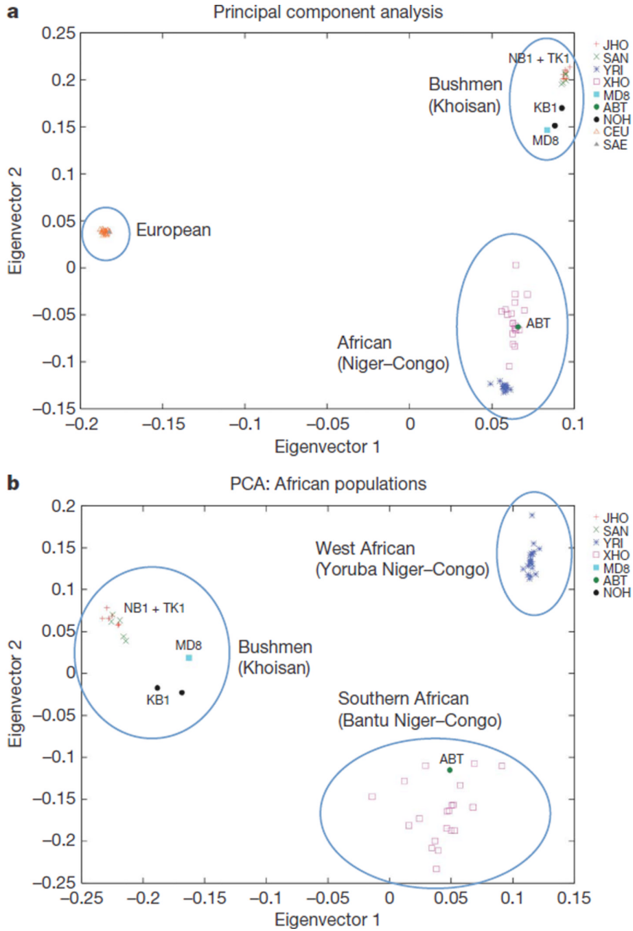
Figure 4. Three-way population structure based on 174,272 autosomal SNPs using PCA a, b , The PCA of Europeans, Africans (Niger-Congo) and Bushmen ( a ) and African populations only ( b ) distinguishes the Bushmen from Yorubans and Bantus. The fraction of the variance explained in a is 0.09 for eigenvector 1 and 0.04 for eigenvector 2, whereas in PCA b it is 0.06 and 0.02, respectively, with a Tracy-Widom P value < 10^{-12} . ABT, sequenced Bantu; CEU, European HapMap; JHO, Juu speakers (including NB1 and TK1); MD8, sequenced !Kung; NOH, Tuu speakers (including KB1); SAE, South African European; SAN, HGDP San; XHO, South African Xhosa; YRI, Yoruba HapMap.
