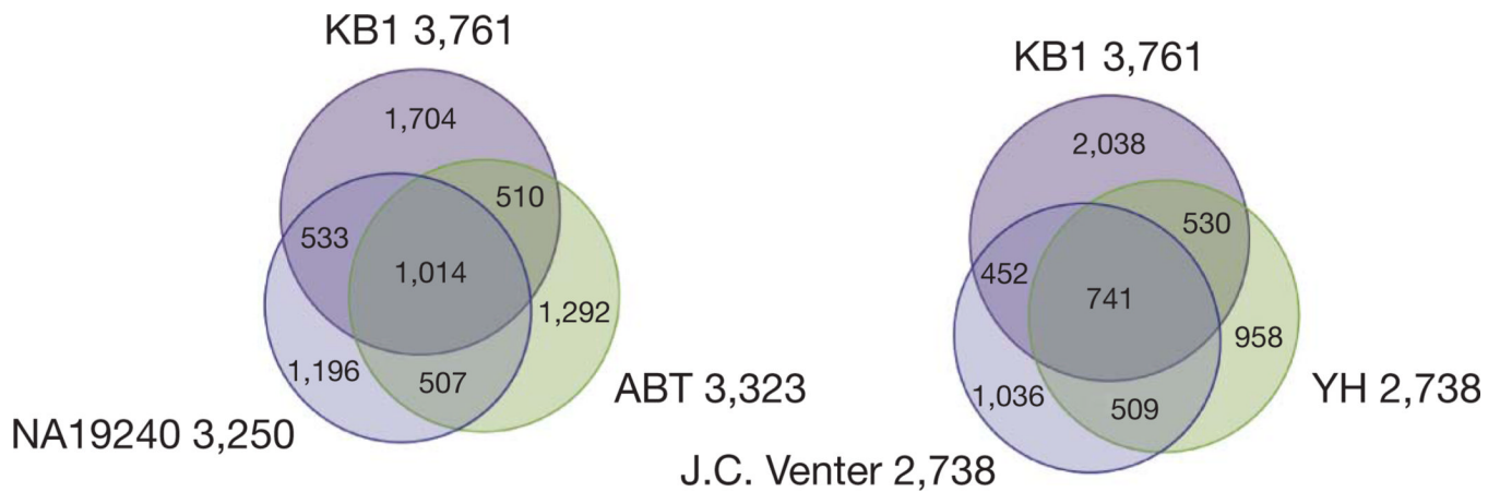
Figure 2. Three-way relationships among SNPs
