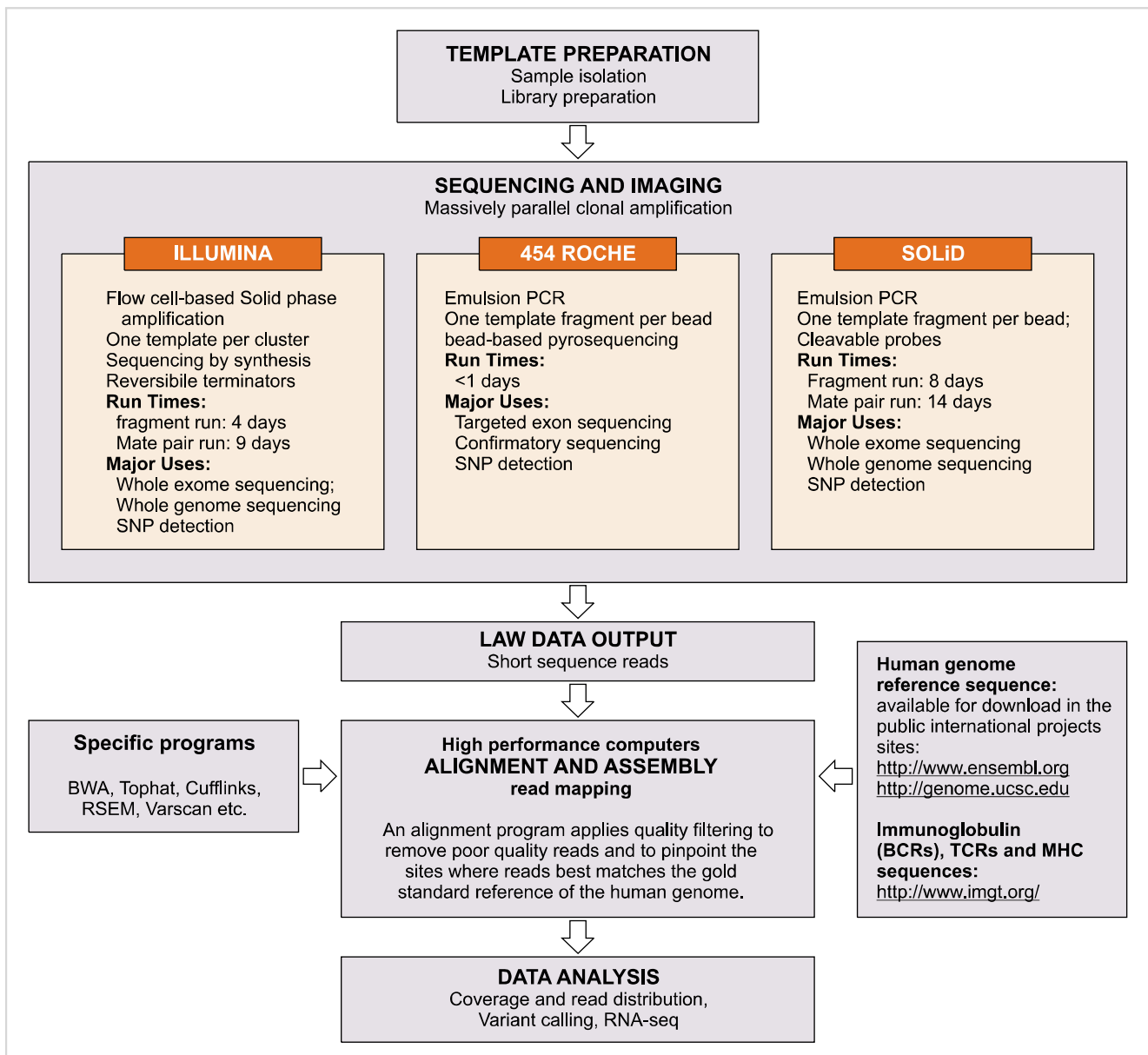
Fig. 1. Next generation sequencing second-generation platforms: comparison and workflow.
