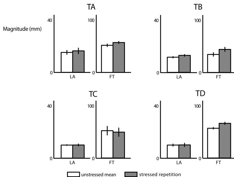
Figure 4. Comparison of the magnitude of repetitions with emphatic stress against the mean magnitude of unstressed repetitions when stress occurs in the opposite domain as the movement. Means and standard deviations shown. There is an overall effect of larger movements under cross-domain stress, but subjects differ slightly in this effect.
