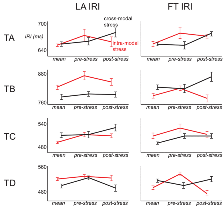
Figure 6. Durational patterns of pre- and post-stress IRIs compared to the mean IRI in positions not adjacent to the emphatic stress. Means and standard deviations shown. All subjects show lengthening of IRIs in stress-adjacent positions in both domains regardless of in which domain the emphatic stress is placed. Subjects differ on the particular implementation of this lengthening.
