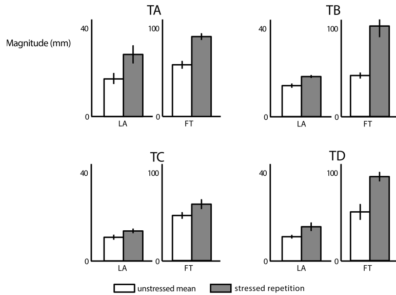
Figure 3. Comparison of the magnitude of repetitions with emphatic stress against the mean magnitude of unstressed repetitions when stress occurs in the same domain as the movement. Means and standard deviations shown. All subjects show larger movements of both lip aperture and fingertip under stress.
