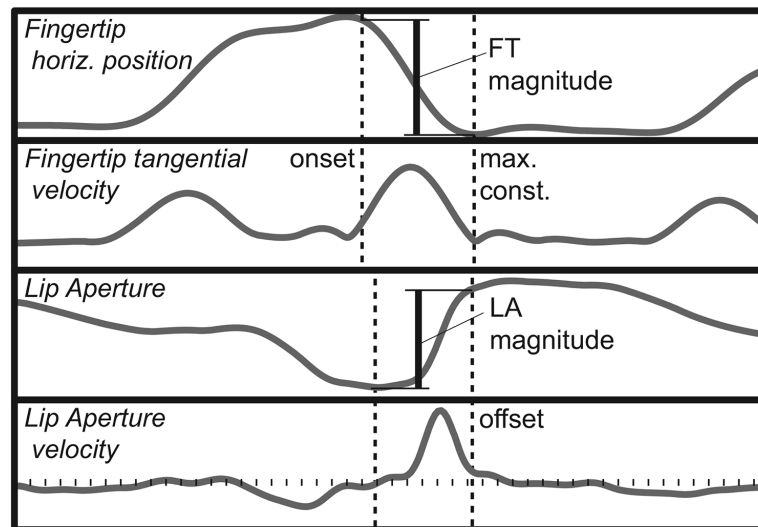
Figure 1. Schematic of measurements taken from articulatory data for lip aperture and Fingertip magnitude. All measurements are based on the zero-crossings in the velocity signal. Fingertip movements are measured from the onset of movement toward the shoulder to the point of maximum constriction. Lip movements measured as the movement from the /m/ to the following vowel.
