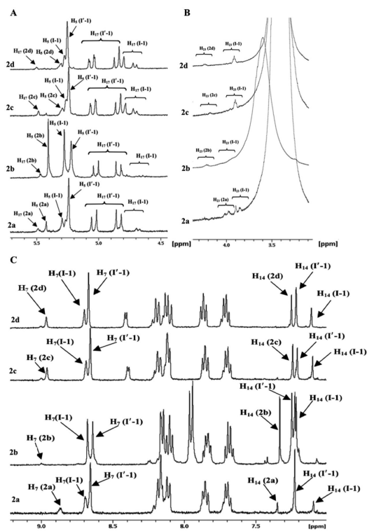
Figure 2. ^1\text{H} NMR spectrum of all four prodrugs in \text{DMSO-}d_6 at 37\text{ }^\circ\text{C} after 6.5 h of incubation in PB pH7.4: (A) section of ^1\text{H} NMR spectrum showing changes in the H-5 and H-17 signals of 2a-d , I-1 , and I0-1 ; (B) section of ^1\text{H} NMR spectrum showing changes in the H-23 signals of 2a-d , and I-1 ; (C) section of ^1\text{H} NMR spectrum showing changes in the H-7 and H-14 signals of 2a-d , I-1 , and I0-1 . Similar spectra were observed at pH 7.0 and 6.6.
