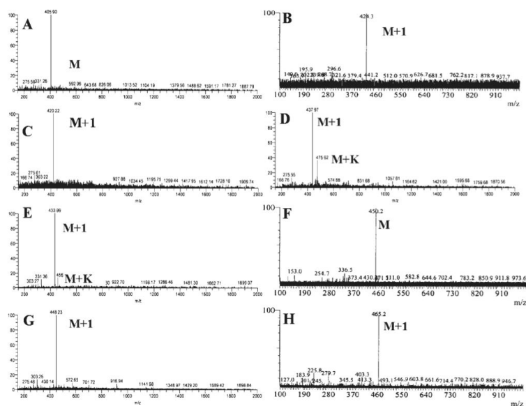
Figure 3. LC-MS spectra of the intermediates obtained during the hydrolysis studies of 2a-d : (A) 2a (I-1) ; (B) 2a (I-2) ; (C) 2b (I-1) ; (D) 2b (I-2) ; (E) 2c (I-1) ; (F) 2c (I-2) ; (G) 2d (I-1) ; (H) 2d (I-2) .
