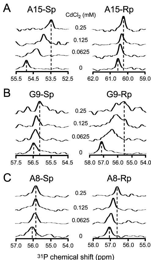
Figure 3. Effect of Cd 2+ ions on the 1D 31 P NMR spectrum of selected SLVI RNAs containing single phosphorothioate modifications. The 1D 31 P spectra of (A) A15-S p and A15-R p , (B) G9-S p and G9-R p , and (C) A8-S p and A8-R p were collected in buffer containing CdCl 2 /MgCl 2 concentrations of 0.0:5.0, 0.0625:4.9375, 0.125:4.875, and 0.25:4.75 mM. Only the most downfield region of the spectra containing the signal from the phosphorothioate is shown.
