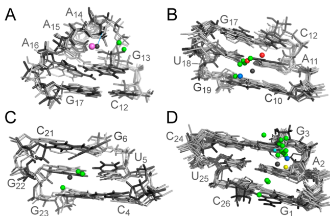
Figure 7. Superposition of metal-binding sites in SLVI with PDB structures containing similar metal-binding sites identified using WebFR3D. The metal-binding sites in SLVI are associated with the (A) GNRA hairpin loop (site 1), (B) C_{10} 5'- PO_4^- (site 2), (C) G_{22} – U_5 wobble (site 4), and (D) 5' end (site 5). The structure and Mg^{2+} ions of SLVI are shown in black, whereas the other structures (PDB entries in Table S2 of Supporting Information) are shown in gray, with their associated metal ion color coded according to the type of metal ( Mg^{2+} , green; Na^+ , purple; Co^{3+} , red; Ca^{2+} , blue; Ni^{2+} , yellow; and Ir^{3+} , light blue).
