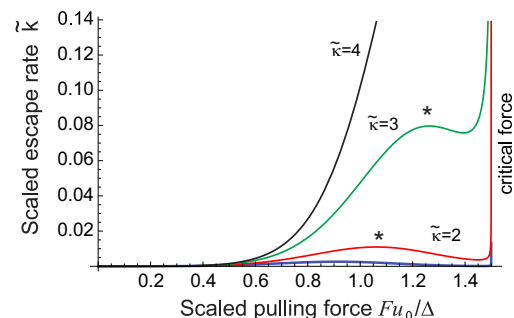
FIGURE 6 The scaled rate of escape as function of the scaled applied pulling force (the same plot as Fig. 5) for a more stiff substrate. The values of \tilde{\kappa} and the position of homeostasis ( F^* ) are labeled on the plot ( lowest barely visible curve is for \tilde{\kappa} = 1 ). On a very stiff substrate, \tilde{\kappa} > 3 , there is a continuous increase in the escape rate of TGF- \beta as the cell applies more force with no homeostatic point F^* (the maximum of k(F) ) present: there is no region of negative feedback in the free TGF- \beta release. The critical force limit F = F_C is at \tilde{f} = 3/2 , at which point the latent complex is ruptured directly. To see this figure in color, go online.
