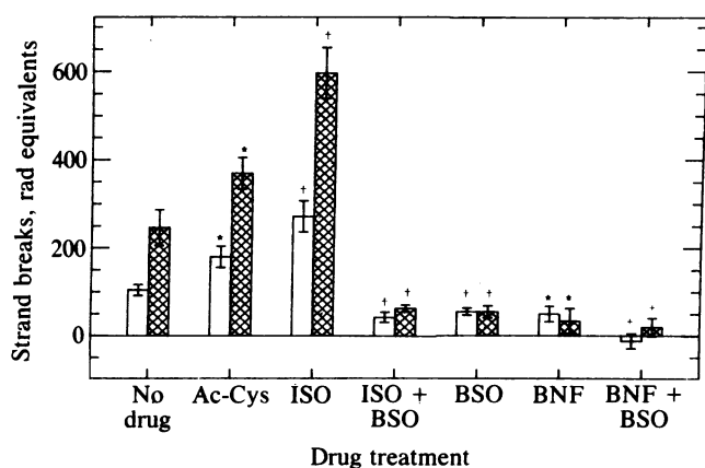
FIG. 1. DNA strand breaks in chicken embryo hepatocytes produced by chromium(VI) after various drug treatments. Cells were pretreated with the indicated drugs and then exposed to 5 \mu M sodium chromate for 2 hr. Ac-Cys, N -acetyl-L-cysteine; ISO, isopentanol; BSO, buthionine sulfoximine; BNF, \beta -naphthoflavone. DNA strand breaks were measured by the alkaline elution technique, without (open bars) or with (cross-hatched bars) proteinase K digestion. Protein-associated strand breaks are represented by the difference between DNA strand breaks with and without proteinase K digestion of the cell lysates. Calculations of DNA damage caused by chromium(VI) treatment compared cells treated with drugs alone with cells treated with chromium(VI) and drugs. Values represent mean \pm SEM for n \geq 6 .
