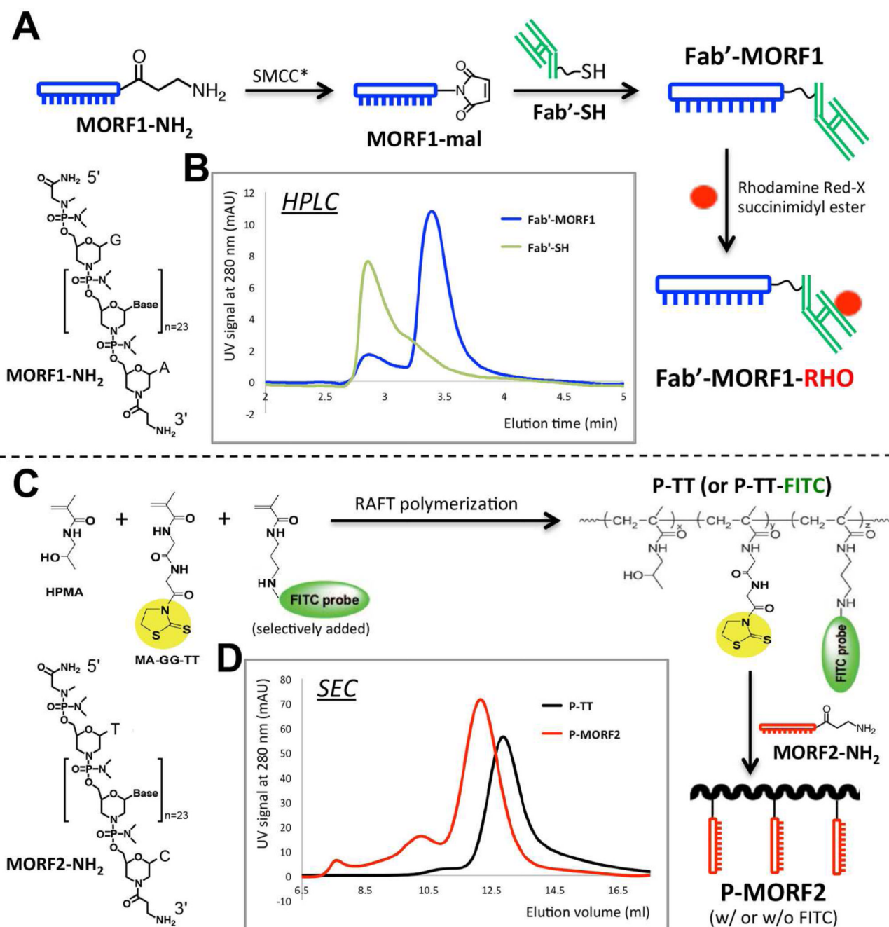
Figure 2. Synthesis and characterization of Fab'-MORF1 and P-MORF2
