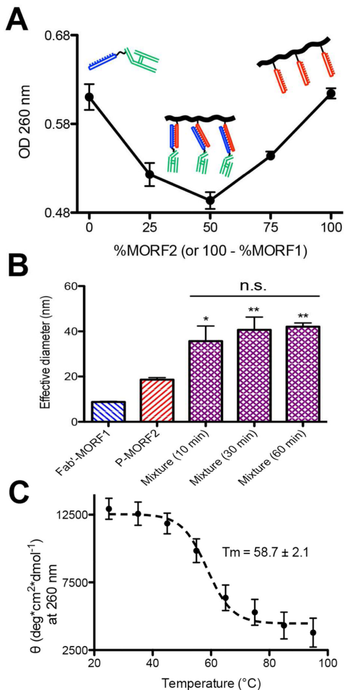
Figure 3. In vitro hybridization of Fab'-MORF1 and P-MORF2
