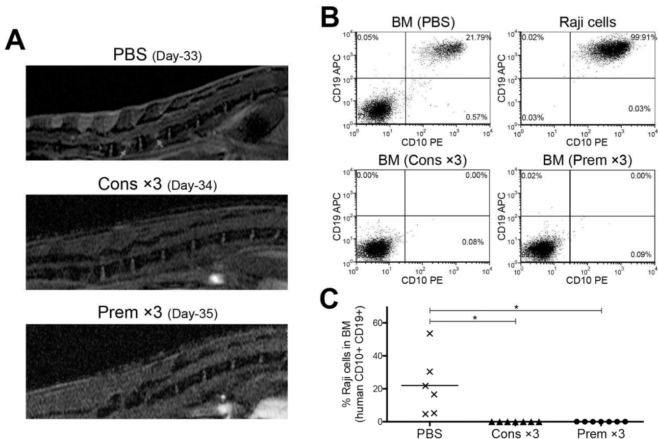
Figure 7. Eradication of Raji cells in SCID mice
