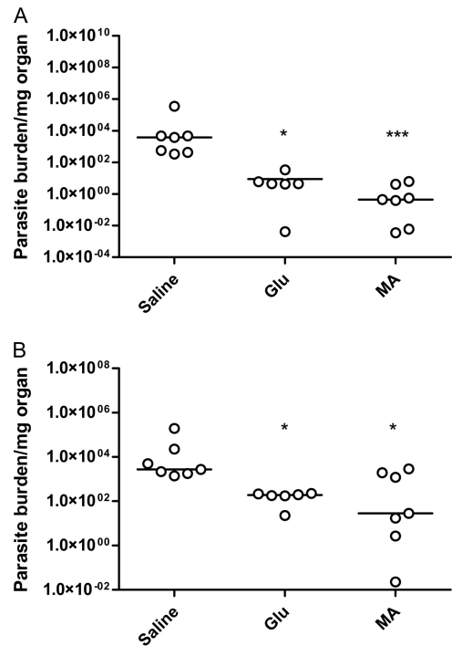
FIG 1 Parasite loads in the livers (A) and spleens (B) of BALB/c mice infected with L. infantum after 20 days of treatment with commercial (Glu) or synthetic meglumine antimoniate (MA) ( 80 \text{ mg} of Sb/kg/day) or saline by the i.p. route. The data are shown as dot plots, and lines correspond to the median of each group ( n = 6 to 7 ). *, P < 0.05 (Kruskal-Wallis, followed by Dunn's multiple-comparison post test).
