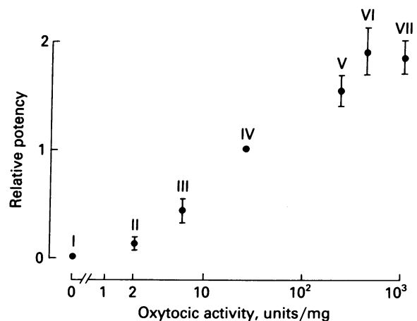
FIG. 3. Relative potency in the hippocampus versus their oxytocic activities of the seven compounds of Table 1. Each point shows the mean increase in firing rate induced by the compounds relative to the increase induced by arginine vasopressin, all applied at 1 \mu\text{M} . SEMs are given (with n \geq 5 ) except for compound IV (arginine vasopressin, serving as internal standard; n = 29 ) and compound I (which was inactive; n = 8 ). Note that relative potency increases with increasing oxytocic activity.
