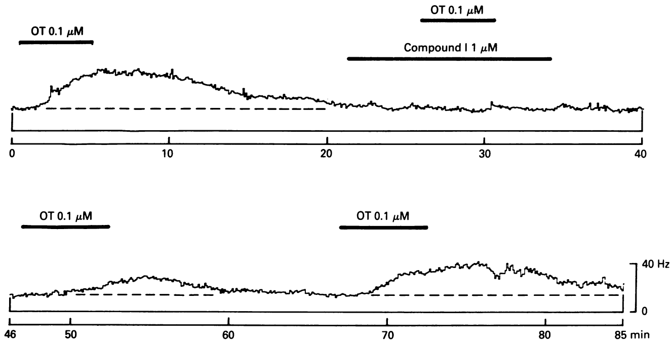
FIG. 5. Reversible antagonism of oxytocin (OT) effect on a CA1 nonpyramidal neuron by a synthetic structural analogue which is an oxytocic and vasopressor antagonist. OT at 0.1 \mu M was applied to the bath (during the periods indicated by thick lines) before, during, and after application of the antagonist 1-deamino-[2-( O -methyltyrosine), 4-valine, 8-D-arginine]vasopressin (compound I) at 1 \mu M. Upper and Lower constitute a continuous rate-meter record except for a 6-min deletion.
