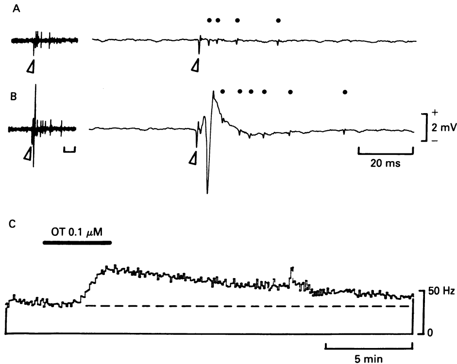
FIG. 1. Characterization of a hippocampal neurone as being nonpyramidal (A and B) and its response to oxytocin (C). A and B illustrate the response of this cell to stimulation of stratum radiatum at two intensities, one subthreshold (A) and the other above threshold (B) for generation of a population response. In A and B, the same response is shown twice: at low speed and under conditions of DC recording (Right) and 5 times faster and filtered (bandwidth, 0.1–3.0 kHz) (Left). Stimulation artefacts are indicated by open arrowheads. Note that stimuli trigger a burst of action potentials marked by black dots (Right), even when subthreshold for elicitation of a population response (A Right). The bursts outlast the duration of the fast, negative component of the population response (B Right), which corresponds to the synchronized discharge of pyramidal neurones. In B, note that the early negative response after the stimulus artefact might contain an early driven action potential, although difficult in this instance to distinguish from the input volley. (C) Rate-meter record shows this spontaneously active neurone to be excited by oxytocin (OT) at 0.1 \mu\text{M} applied during the period indicated by the thick horizontal line.
