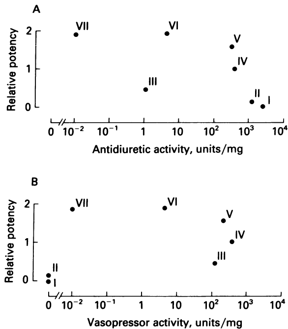
FIG. 4. Relative potency versus antidiuretic (A) or vasopressor (B) activities described in Table 1 (second and third columns). SEMs, being the same as in Fig. 2, have been omitted for clarity. Note the lack of correlation between the potency of these seven compounds in hippocampus and their activity as antidiuretic or vasopressor agonists (e.g., compound VII, which virtually lacks any vasopressor or antidiuretic activity, is an extremely potent agonist in the hippocampus).
