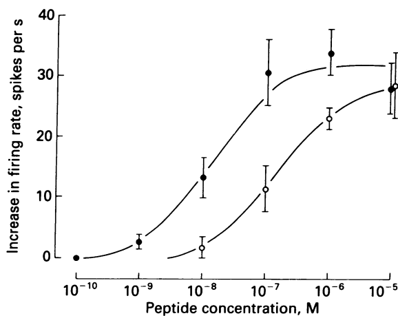
FIG. 2. Effects of oxytocin (●) and arginine vasopressin (○) applied at various concentrations on the firing of nonpyramidal neurones. Each point shows the mean increase [ \pm SEM ( n = 5 ) except for oxytocin at 1 \mu\text{M} , where n = 13 , and arginine vasopressin at 1 \mu\text{M} , where n = 23 ] in firing rate at the concentration of peptide indicated. Oxytocin at 0.1 nM never had an effect; consequently, this point has no SEM.
