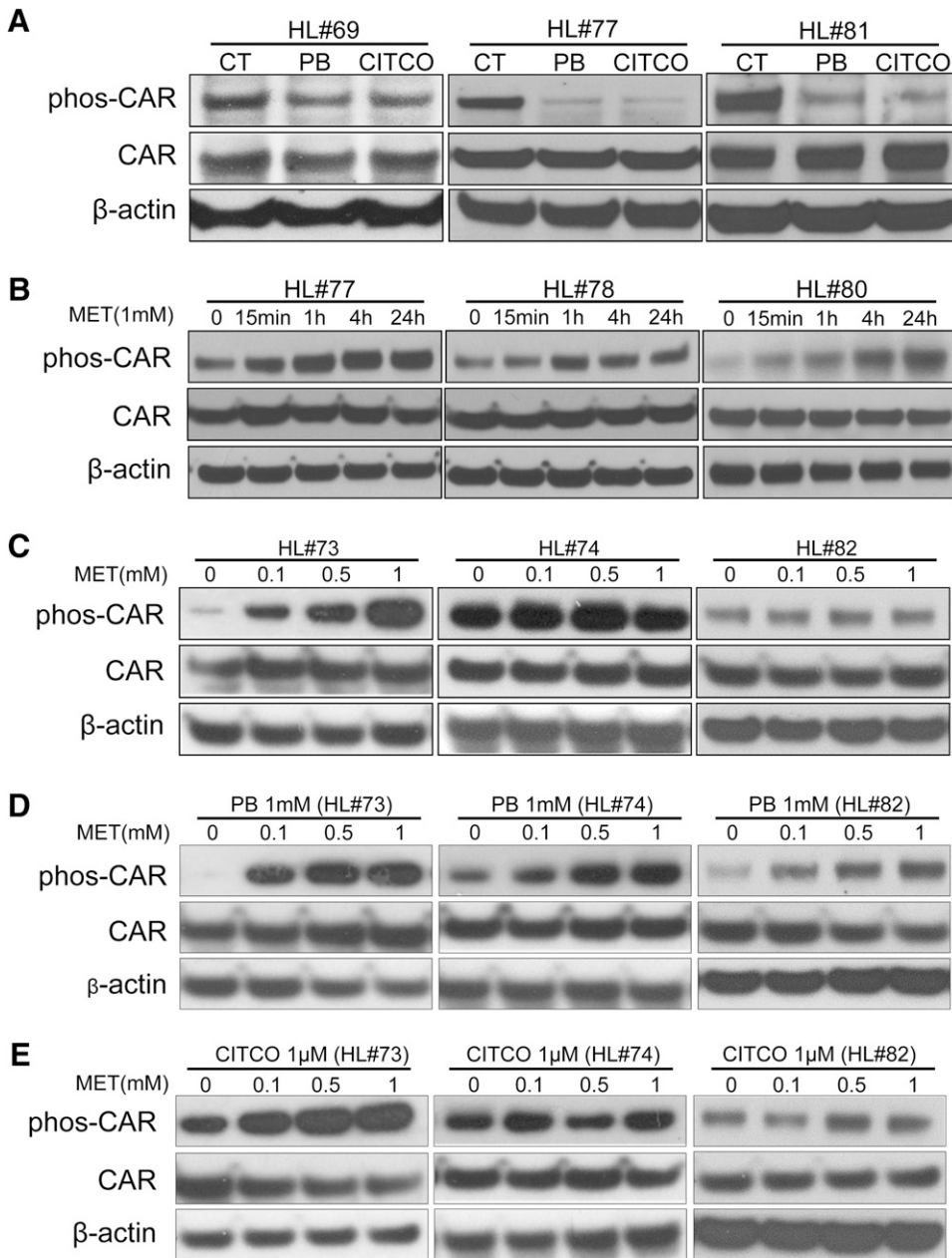
Fig. 4. Metformin enhances phosphorylation of CAR. Homogenate proteins from treated human hepatocytes were used for Western blot analysis of phosphorylated Thr38 hCAR, total hCAR, and \beta -actin as described in Materials and Methods . Specific treatments in this study include (A) DMSO (0.1%), PB (1 mM), or CITCO (1 \mu M) for 24 hours in human hepatocytes (HL#69, #77, and #81); (B) MET (1 mM) for 0, 15 minutes, 1 hour, 4 hours, and 24 hours in human hepatocytes (HL#77, #78, and #80); (C) MET (0.1, 0.5, 1 mM); and the combination of (D) MET with PB (1 mM) or (E) CITCO (1 \mu M) for 24 hours in human hepatocytes (HL#73, #74, and #82).
