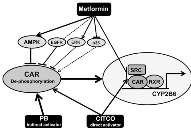
Fig. 8. Model of metformin-mediated CAR phosphorylation and de-activation. The schematic figure illustrates that metformin inhibits both the nuclear translocation and nuclear activation of CAR, and represses CYP2B6 expression induced by PB and CITCO. In the cytoplasm, metformin enhances CAR phosphorylation thereby blocks its nuclear translocation, primarily through the AMPK and ERK1/2 pathways, with the p38 MAPK and EGFR signaling negligibly involved. Inside the nucleus, metformin can disrupt the interaction between CAR and coactivators, which was enhanced by the direct hCAR activator CITCO. The solid and dashed lines indicate strong and weak interactions, respectively. The arrows show activation and the blunt-head lines demonstrate inhibition.
