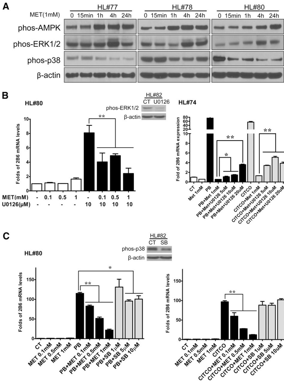
Fig. 6. ERK1/2 and p38 MAPK signaling in metformin-mediated CAR phosphorylation. Human hepatocytes (HL#77, #78, and #80) were treated with MET (1 mM) for 0, 15 minutes, and 1, 4, and 24 hours. Homogenate proteins from each treatment group were used for Western blot analysis of AMPK (Thr172), ERK1/2 (Thr202/Tyr204), p38 MAPK (Thr180/Tyr182), and \beta -actin (A). Real-time PCR was employed to measure CYP2B6 expression in human hepatocytes (HL#74 and #80) treated for 24 hours with 0.1% DMSO, MET (0.1, 0.5, 1 mM), U0126 (10 \mu M), PB (1 mM), CITCO (1 \mu M), SB212190 (1, 5, 10 \mu M), or their different combinations as indicated in B and C. Dephosphorylation of ERK1/2 by U0126 (10 \mu M) and p38 MAPK by SB212190 (10 \mu M) were analyzed in treated hepatocytes (HL#82). Data represent the mean \pm S.D. of three independent transfections (* P < 0.05; ** P < 0.01).
