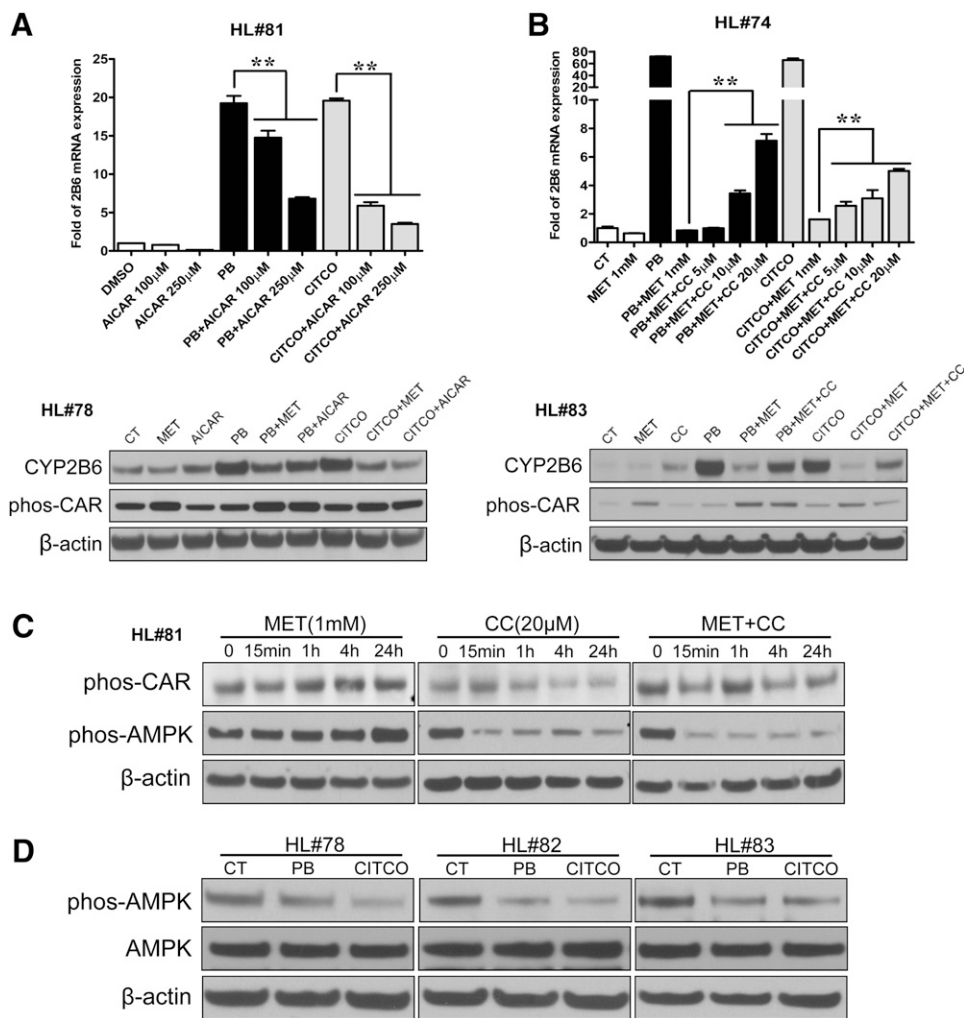
Fig. 5. Metformin promotes CAR phosphorylation by activating AMPK. (A) Human hepatocytes (HL#78 and #81) were treated with DMSO (0.1%), AICAR (100, 250 μM), PB (1 mM), CITCO (1 μM), or their combinations as indicated. CYP2B6 expression was assayed by real-time PCR and Western blot analysis. (B) Human hepatocytes (HL#74 and #83) were treated with 0.1% DMSO, PB (1 mM), CITCO (1 μM), MET (1 mM), Compound C (CC; 5, 10, 20 μM), or their combinations as outlined in Materials and Methods . Total RNA from each group was analyzed by real-time PCR for CYP2B6 expression. Homogenate proteins from each treated hepatocytes were used for Western blot analysis of CYP2B6, hCAR (Thr38), and β-actin. (C) Human hepatocytes (HL#81) were treated with MET (1 mM), CC (20 μM), or their combination for 0, 15 minutes, and 1, 4, and 24 hours. Homogenate proteins from treated hepatocytes were used for Western blot analysis of hCAR (Thr38), AMPK (Thr172), and β-actin. (D) Phosphorylation of AMPK (Thr172) was also measured in human hepatocytes (HL#78, #82, and #83) after the treatment of vehicle control (0.1% DMSO), PB (1 mM), or CITCO (1 μM) for 24 hours. Data represent the mean ± S.D. of three independent transfections (** P < 0.01).
