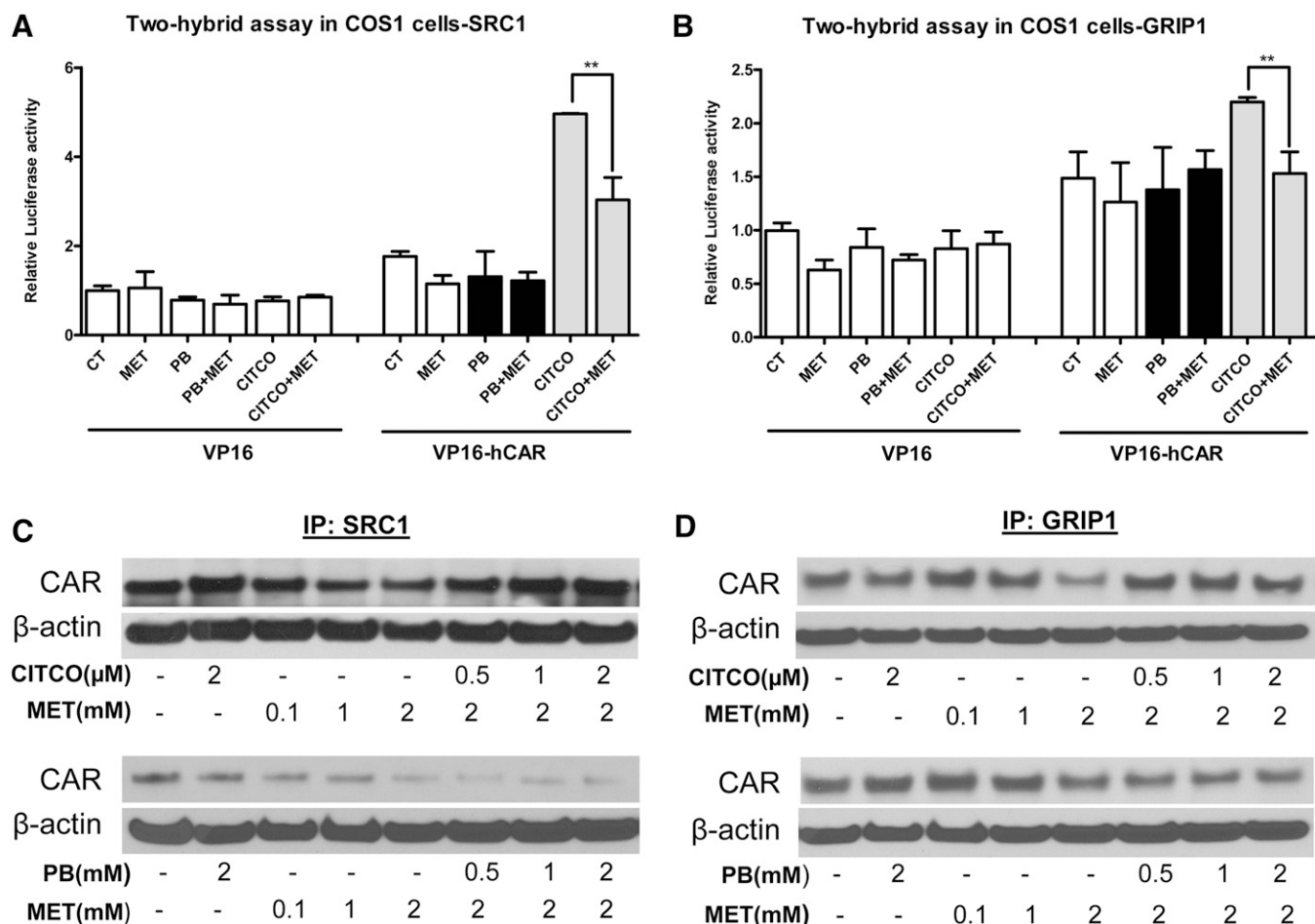
Fig. 3. Metformin disrupts interaction between hCAR and coactivators. Mammalian two-hybrid assays were performed in COS1 cells transfected with expression plasmids encoding VP16-AD/hCAR fusion proteins and GAL4-DBD/coactivator fusion proteins as indicated—(A) SRC1, and (B) GRIP1—together with the reporter gene plasmid pG5luc for 16 hours. Cells were treated with vehicle control (0.1% DMSO), PB (1 mM), CITCO (1 \mu M), MET (1 mM), or their combination for another 24 hours before the determination of luciferase activities. Data represent the mean \pm S.D. of three independent transfections (** P < 0.01 ). Coimmunoprecipitation assays were performed using COS7 cells transfected with expression plasmids encoding hCAR and coactivator proteins: (C) SRC1 and (D) GRIP1. The whole cell lysate was collected and incubated with DMSO (0.1%), MET (0.1, 1.0, 2.0 mM), PB (0.5, 1, 2 mM), CITCO (0.5, 1.0, 2.0 \mu M), or their combination overnight at 4°C. Proteins were immunoprecipitated and analyzed by Western blot analysis as outlined in Materials and Methods .
