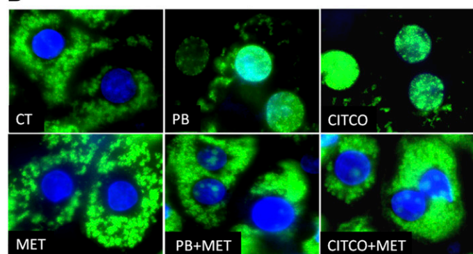
Fig. 2. Metformin suppresses CAR activation in human primary hepatocytes. (A) Human primary hepatocytes (HL#74 and #80) were transfected with the CYP2B6 reporter and the pRL-TK plasmids using Effectene reagent as described in Materials and Methods . Subsequently, transfected hepatocytes were treated with DMSO (0.1%), MET (1 mM), PB (1 mM), CITCO (1 \mu M), or their combinations for 24 hours before the determination of luciferase activities. Data represent the mean \pm S.D. of three independent transfections (* P < 0.05; ** P < 0.01). (B) Human hepatocytes were infected with Ad/EYFP-hCAR for 24 hours followed by treatment with DMSO (0.1%), MET (1 mM), PB (1 mM), CITCO (1 \mu M), or their combinations as indicated for 12 hours. Confocal images of hepatocytes from a representative donor (HL#77) were shown for the localization and translocation of EYFP-hCAR. Over 100 EYFP-hCAR-expressing cells per treatment group were counted and classified as cytosolic, nuclear, or mixed (cytosolic and nuclear) cellular localizations.
