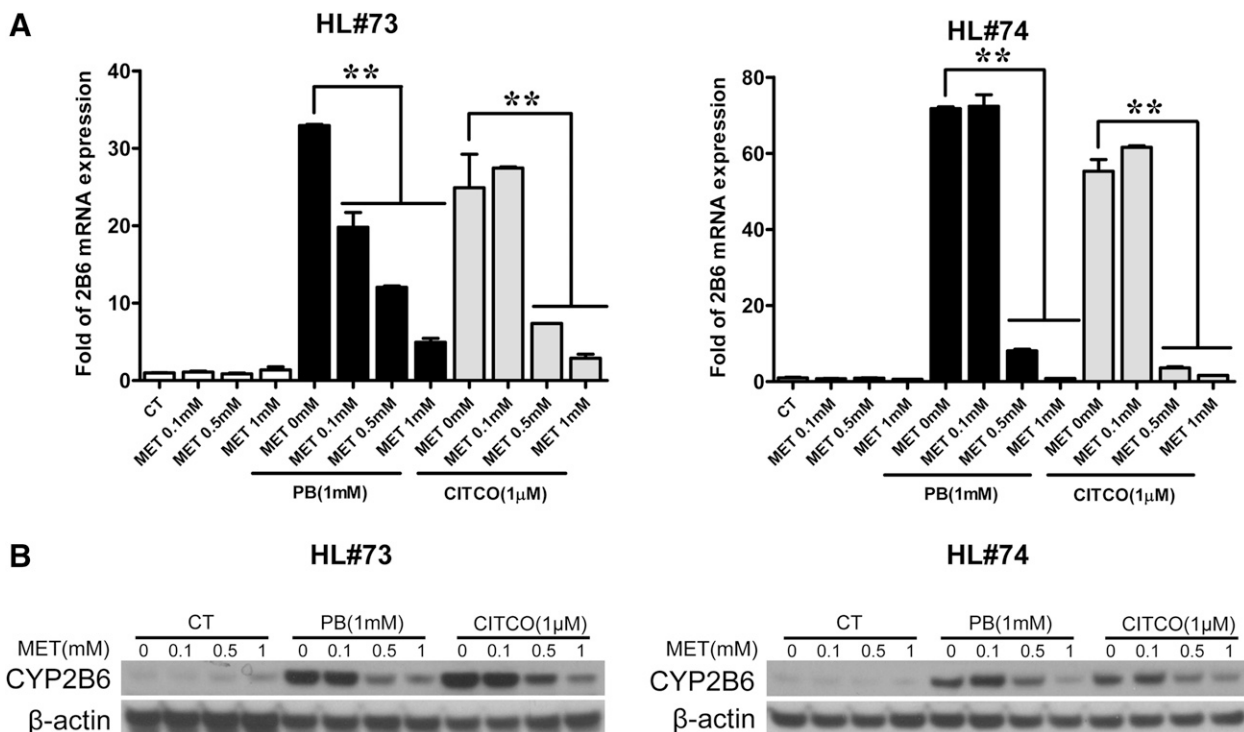
Fig. 1. Metformin represses PB and CITCO induced CYP2B6 expression. Human hepatocytes (HL#73 and #74) were treated with vehicle control (CT; 0.1% DMSO), PB (1 mM), CITCO (1 \mu M), MET (0.1, 0.5, 1 mM), or their combinations as indicated for 24 hours or 72 hours for analysis of mRNA and protein expression, respectively. Total RNA extracted from hepatocytes was subjected to real-time PCR analysis of CYP2B6 expression (A). Homogenate proteins (20 \mu g) from each group were prepared for CYP2B6 and \beta -actin immunoblotting analysis (B). Data represent the mean \pm S.D. of three independent transfections (** P < 0.01 ).
